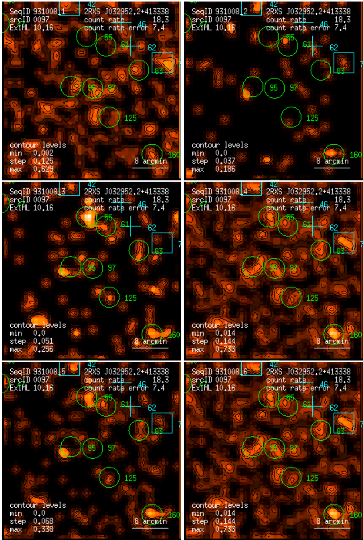
Figure 97: RASS 931008: detection 0097: band rate images, Gaussian filter: (1) PSPC channels 11 – 41, (2) 52 – 90, (3) 91 – 201, (4) 11 – 235, (5) 52 – 201, (6) 11 – 201. Broad band rates in counts/ks. Band rate contour levels in counts/ks/arcmin 2 .
