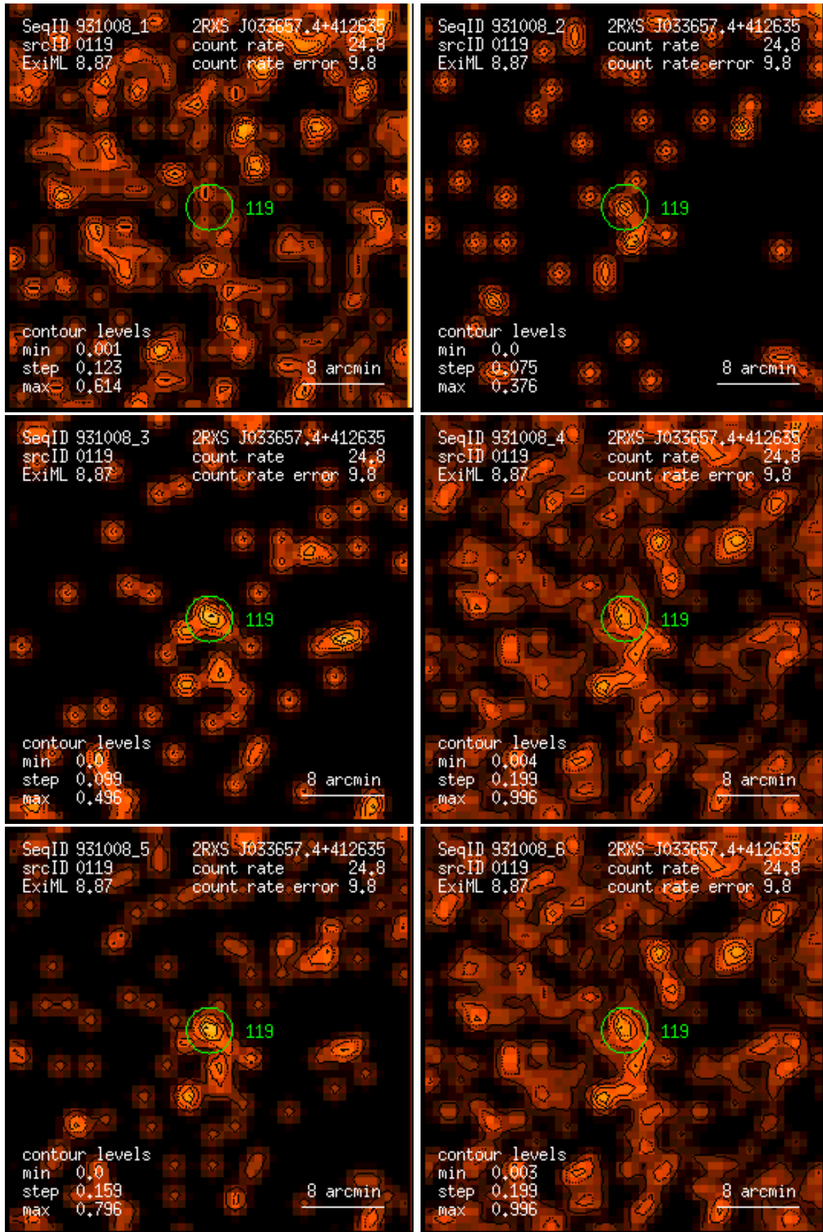
Figure 119: RASS 931008: detection 0119: band rate images, Gaussian filter: (1) PSPC channels 11 – 41, (2) 52 – 90, (3) 91 – 201, (4) 11 – 235, (5) 52 – 201, (6) 11 – 201. Broad band rates in counts/ks. Band rate contour levels in counts/ks/arcmin 2 .
