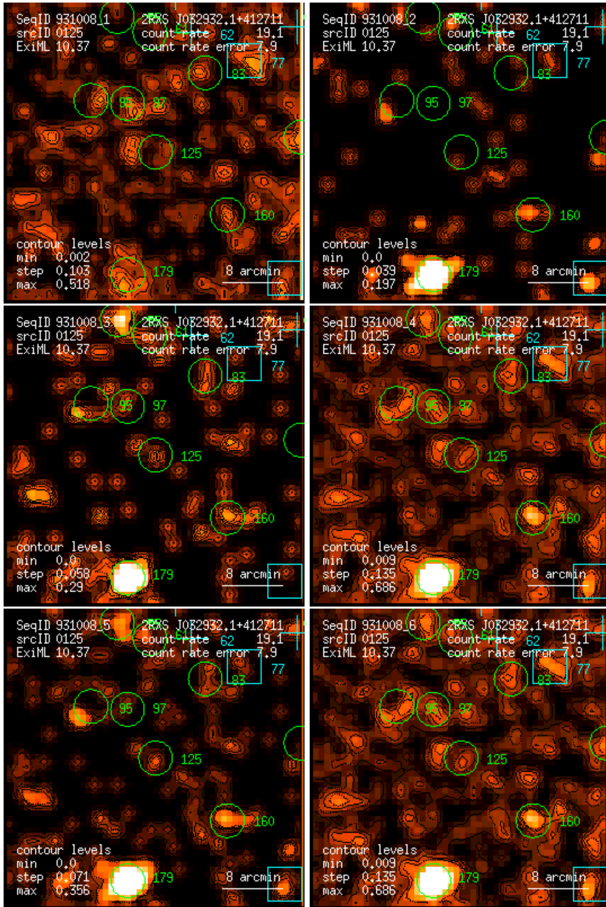
Figure 125: RASS 931008: detection 0125: band rate images, Gaussian filter: (1) PSPC channels 11 – 41, (2) 52 – 90, (3) 91 – 201, (4) 11 – 235, (5) 52 – 201, (6) 11 – 201. Broad band rates in counts/ks. Band rate contour levels in counts/ks/arcmin 2 .
