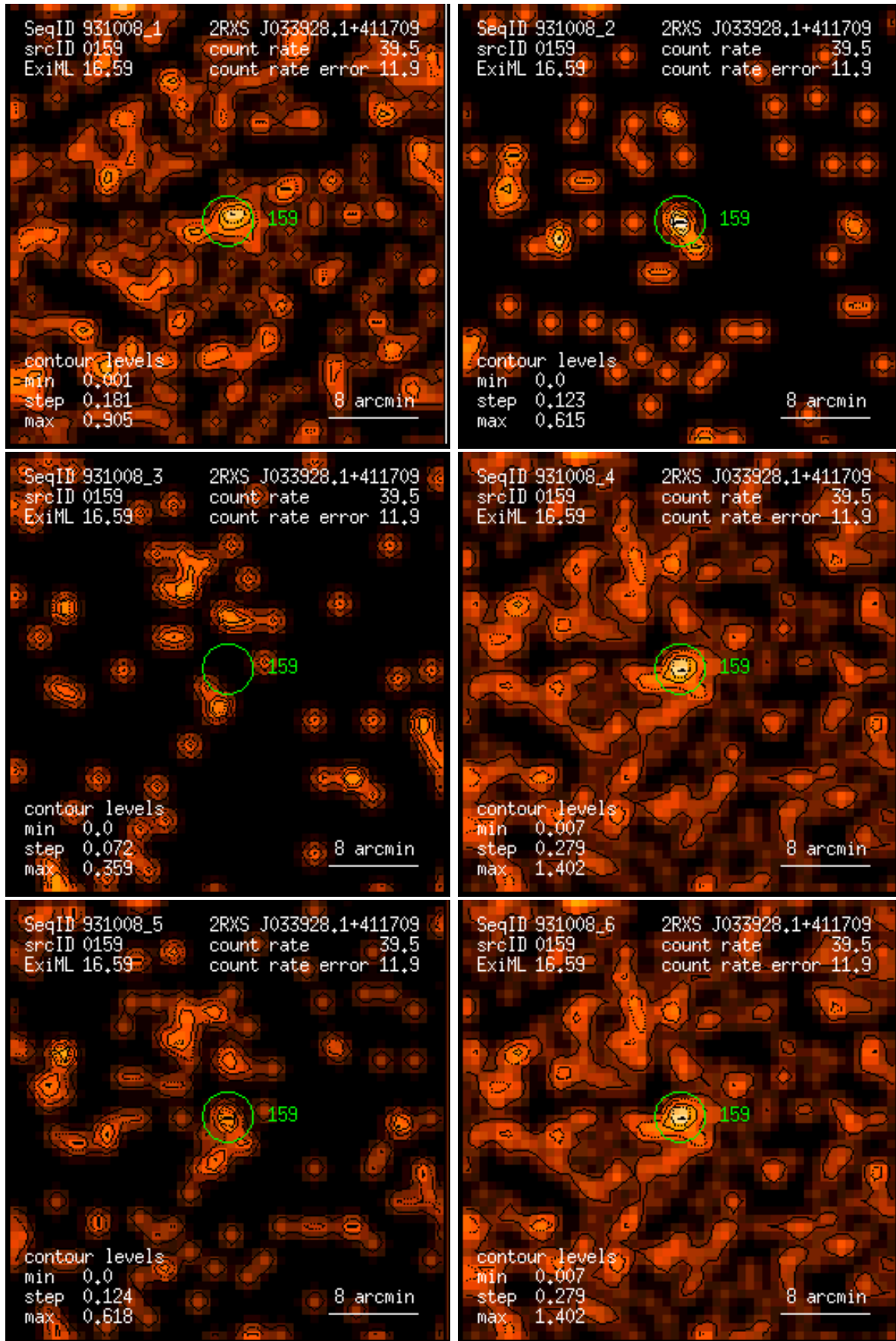
Figure 159: RASS 931008: detection 0159: band rate images, Gaussian filter: (1) PSPC channels 11 – 41, (2) 52 – 90, (3) 91 – 201, (4) 11 – 235, (5) 52 – 201, (6) 11 – 201. Broad band rates in counts/ks. Band rate contour levels in counts/ks/arcmin 2 .
