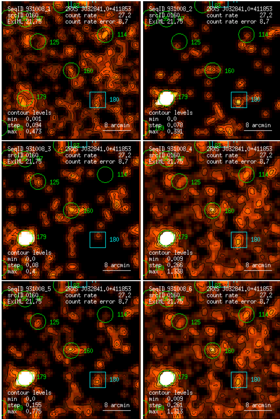
Figure 160: RASS 931008: detection 0160: band rate images, Gaussian filter: (1) PSPC channels 11 – 41, (2) 52 – 90, (3) 91 – 201, (4) 11 – 235, (5) 52 – 201, (6) 11 – 201. Broad band rates in counts/ks. Band rate contour levels in counts/ks/arcmin 2 .
