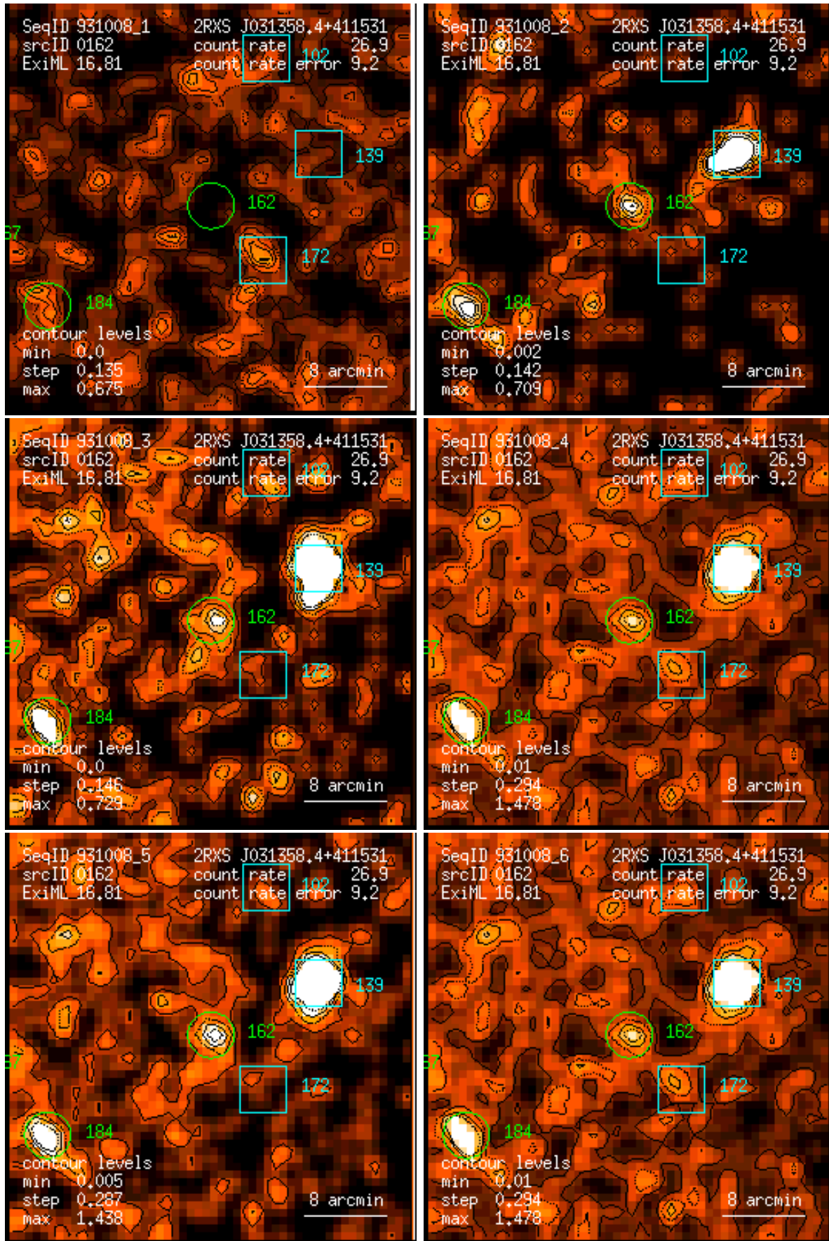
Figure 162: RASS 931008: detection 0162: band rate images, Gaussian filter: (1) PSPC channels 11 – 41, (2) 52 – 90, (3) 91 – 201, (4) 11 – 235, (5) 52 – 201, (6) 11 – 201. Broad band rates in counts/ks. Band rate contour levels in counts/ks/arcmin 2 .
