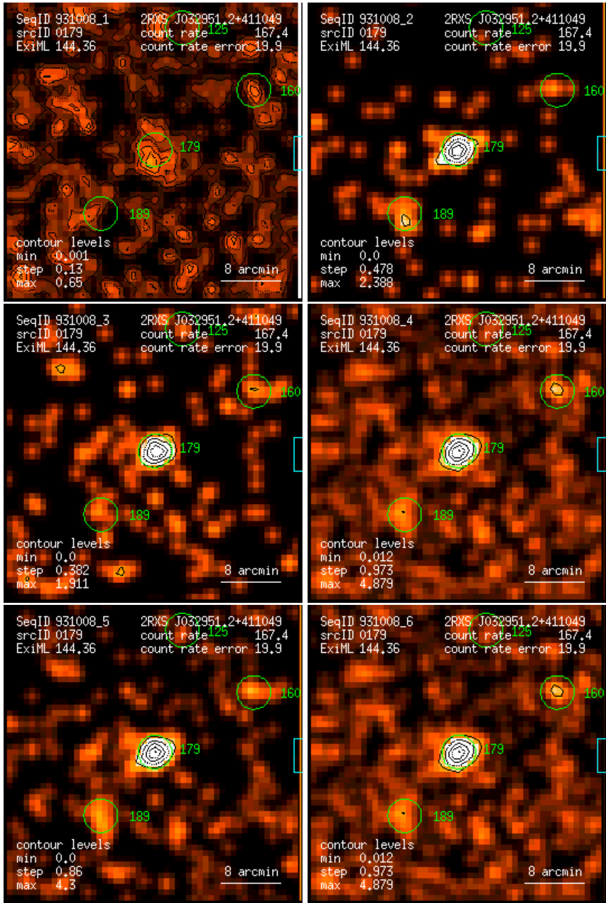
Figure 179: RASS 931008: detection 0179: band rate images, Gaussian filter: (1) PSPC channels 11 – 41, (2) 52 – 90, (3) 91 – 201, (4) 11 – 235, (5) 52 – 201, (6) 11 – 201. Broad band rates in counts/ks. Band rate contour levels in counts/ks/arcmin 2 .
