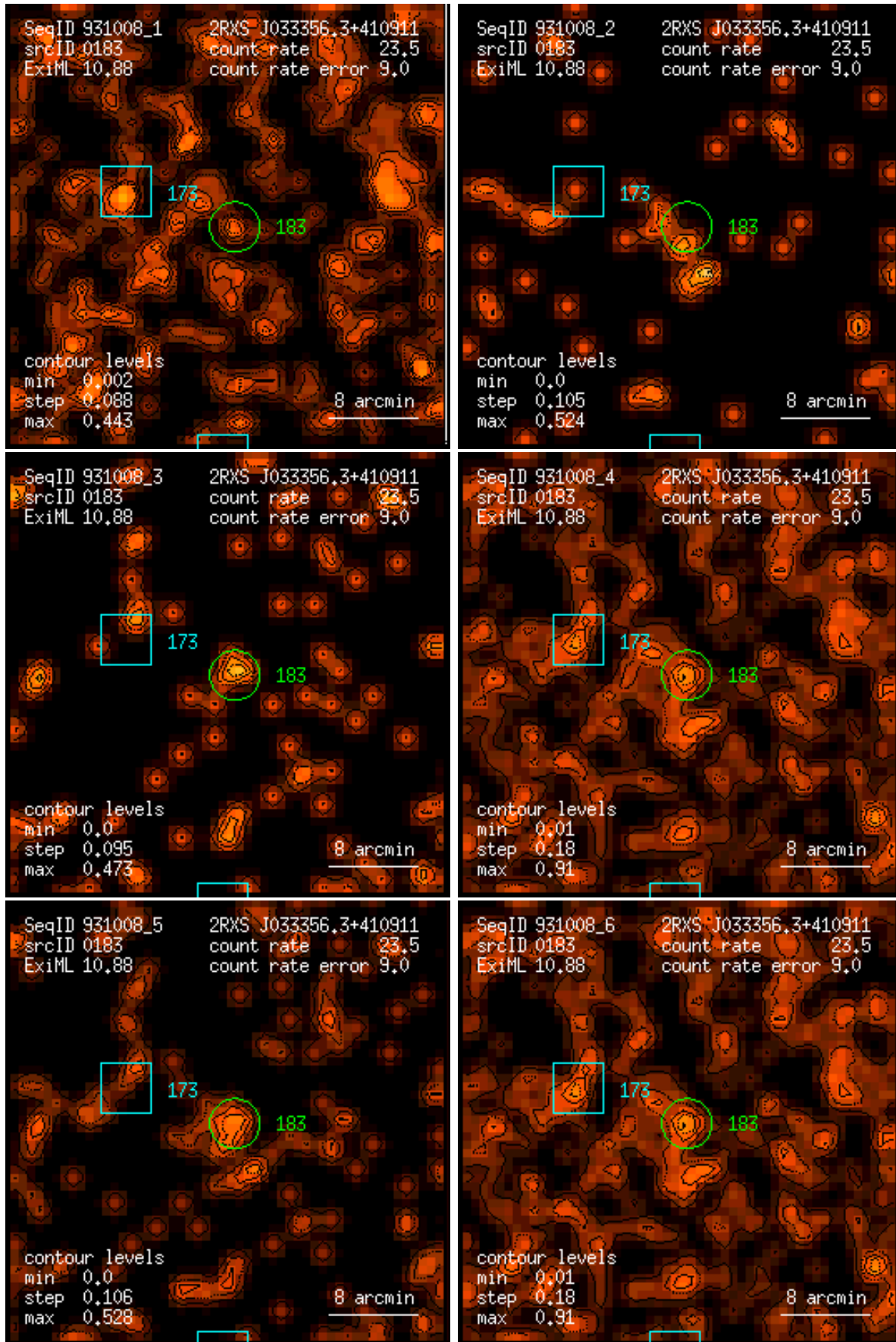
Figure 183: RASS 931008: detection 0183: band rate images, Gaussian filter: (1) PSPC channels 11 – 41, (2) 52 – 90, (3) 91 – 201, (4) 11 – 235, (5) 52 – 201, (6) 11 – 201. Broad band rates in counts/ks. Band rate contour levels in counts/ks/arcmin 2 .
