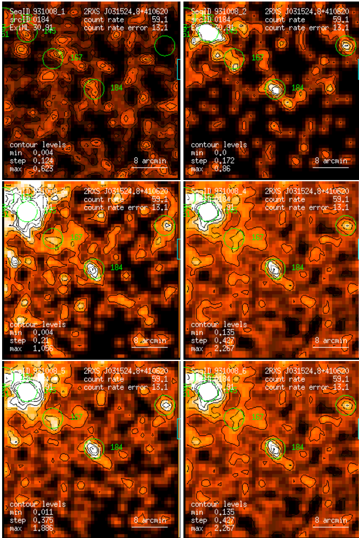
Figure 184: RASS 931008: detection 0184: band rate images, Gaussian filter: (1) PSPC channels 11 – 41, (2) 52 – 90, (3) 91 – 201, (4) 11 – 235, (5) 52 – 201, (6) 11 – 201. Broad band rates in counts/ks. Band rate contour levels in counts/ks/arcmin 2 .
