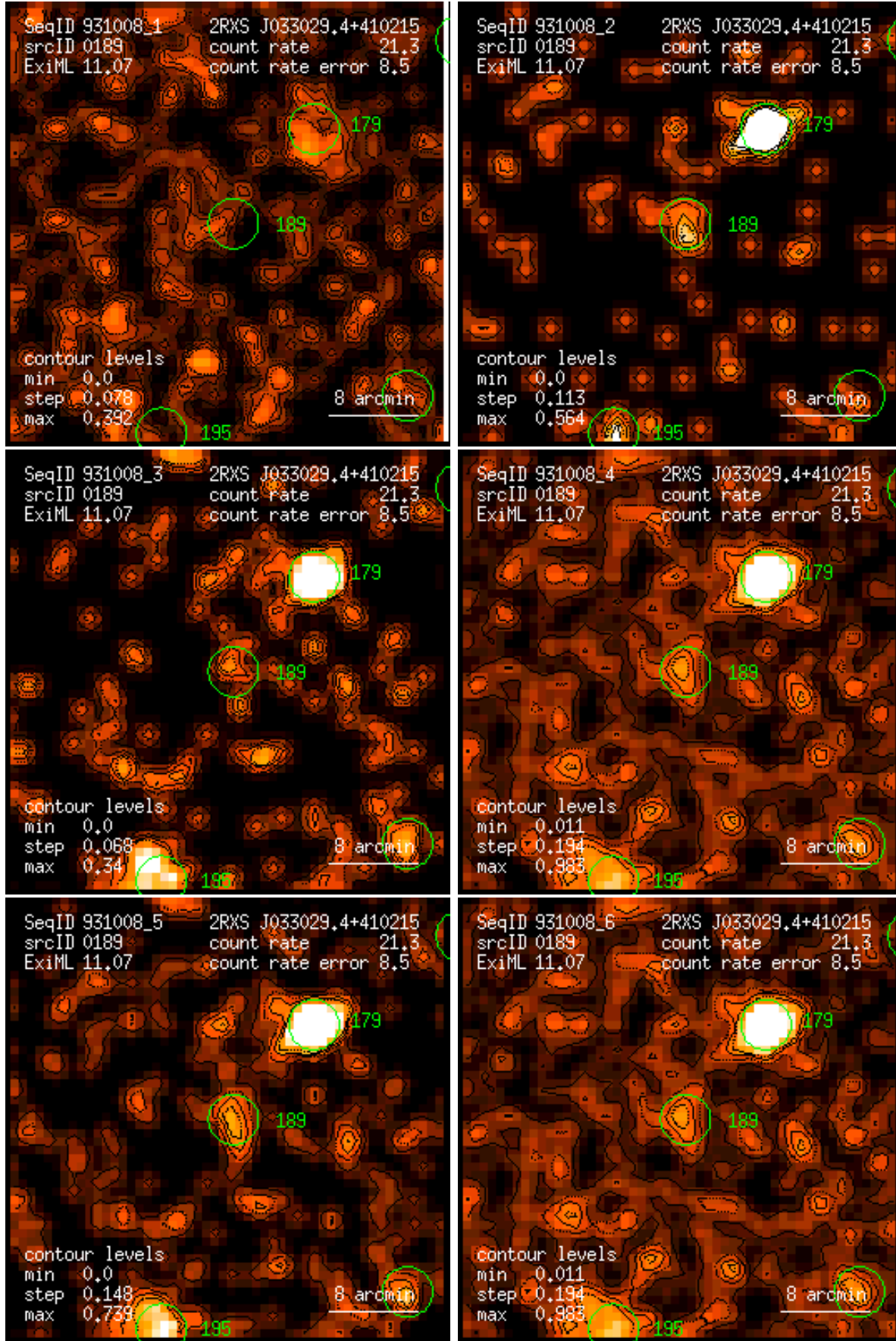
Figure 189: RASS 931008: detection 0189: band rate images, Gaussian filter: (1) PSPC channels 11 – 41, (2) 52 – 90, (3) 91 – 201, (4) 11 – 235, (5) 52 – 201, (6) 11 – 201. Broad band rates in counts/ks. Band rate contour levels in counts/ks/arcmin 2 .
