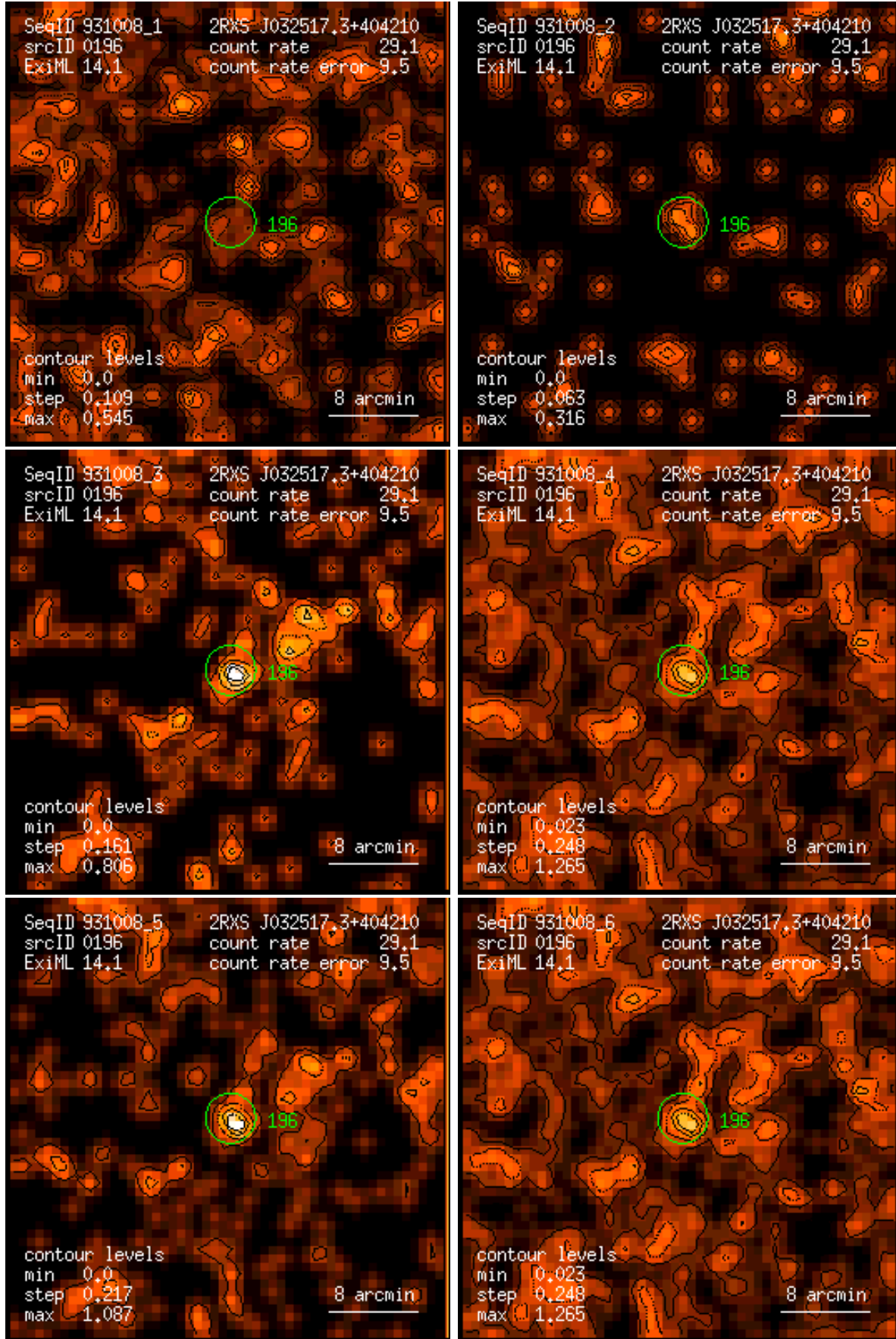
Figure 196: RASS 931008: detection 0196: band rate images, Gaussian filter: (1) PSPC channels 11 – 41, (2) 52 – 90, (3) 91 – 201, (4) 11 – 235, (5) 52 – 201, (6) 11 – 201. Broad band rates in counts/ks. Band rate contour levels in counts/ks/arcmin 2 .
