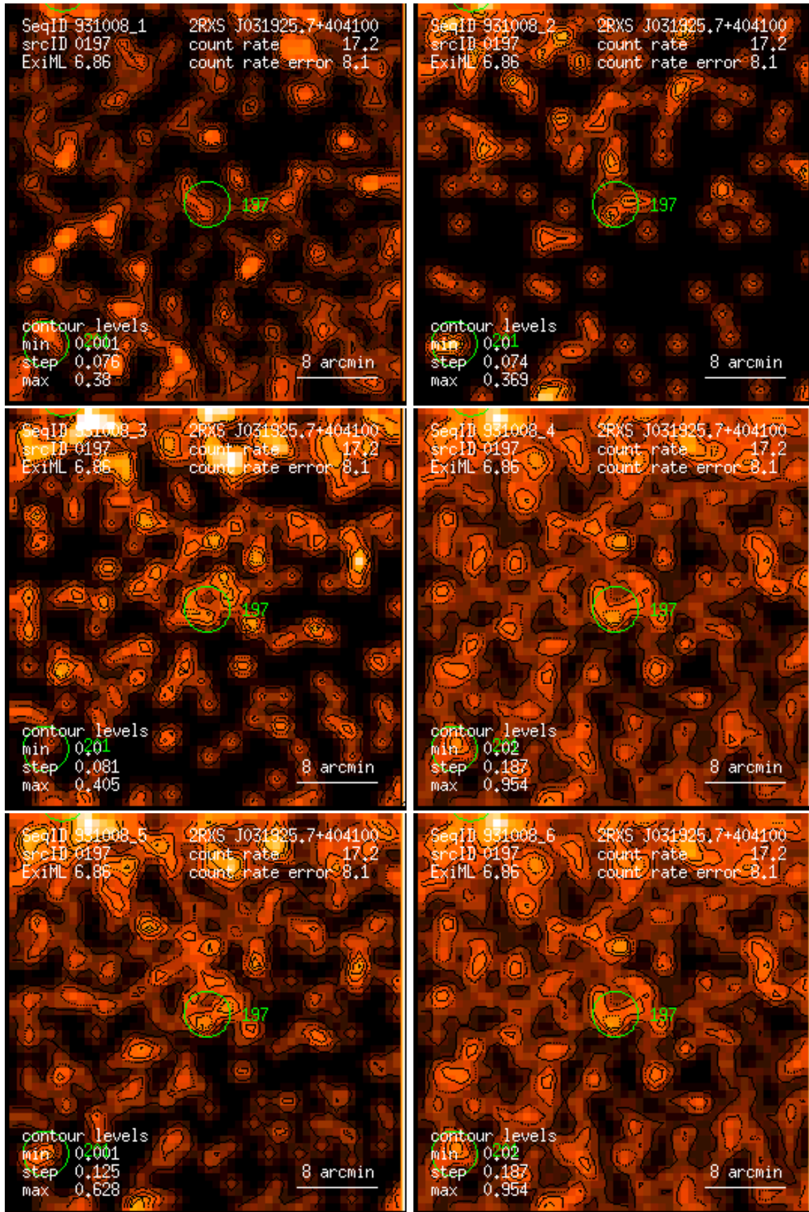
Figure 197: RASS 931008: detection 0197: band rate images, Gaussian filter: (1) PSPC channels 11 – 41, (2) 52 – 90, (3) 91 – 201, (4) 11 – 235, (5) 52 – 201, (6) 11 – 201. Broad band rates in counts/ks. Band rate contour levels in counts/ks/arcmin 2 .
