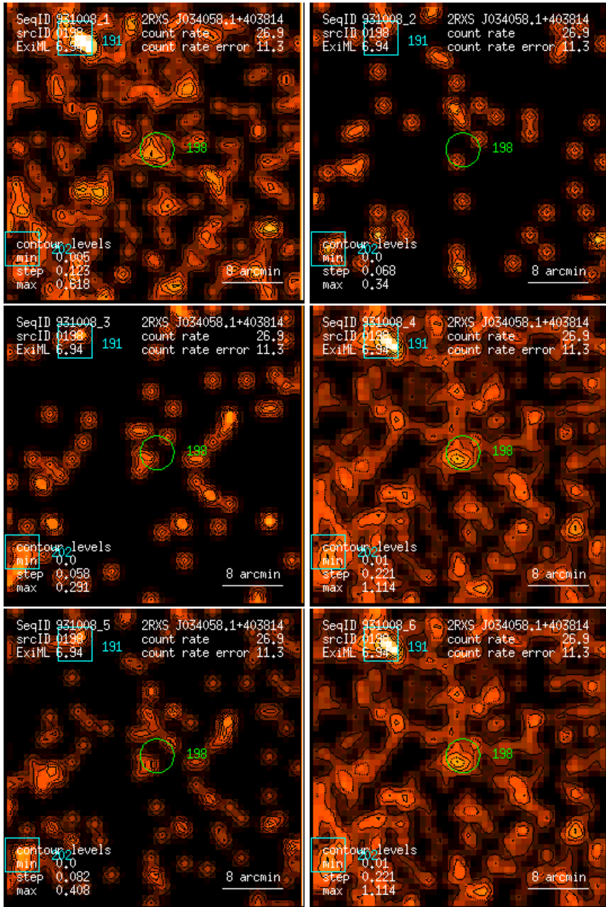
Figure 198: RASS 931008: detection 0198: band rate images, Gaussian filter: (1) PSPC channels 11 – 41, (2) 52 – 90, (3) 91 – 201, (4) 11 – 235, (5) 52 – 201, (6) 11 – 201. Broad band rates in counts/ks. Band rate contour levels in counts/ks/arcmin 2 .
