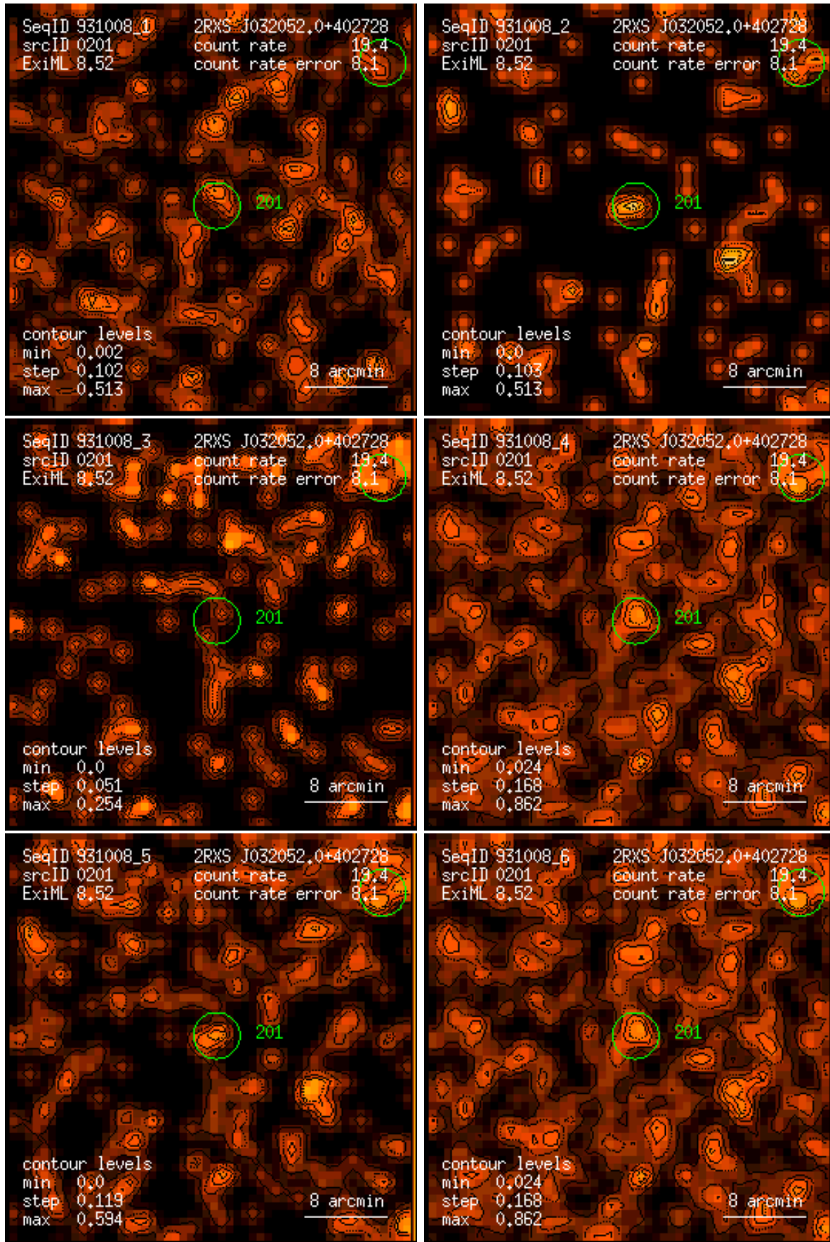
Figure 201: RASS 931008: detection 0201: band rate images, Gaussian filter: (1) PSPC channels 11 – 41, (2) 52 – 90, (3) 91 – 201, (4) 11 – 235, (5) 52 – 201, (6) 11 – 201. Broad band rates in counts/ks. Band rate contour levels in counts/ks/arcmin 2 .
