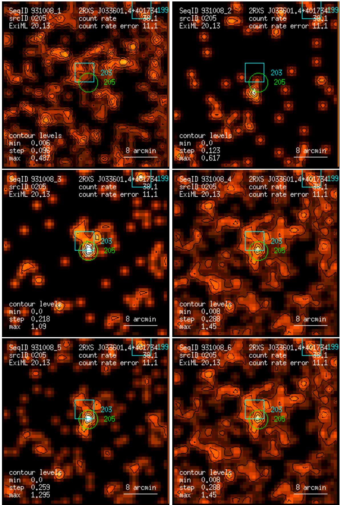
Figure 205: RASS 931008: detection 0205: band rate images, Gaussian filter: (1) PSPC channels 11 – 41, (2) 52 – 90, (3) 91 – 201, (4) 11 – 235, (5) 52 – 201, (6) 11 – 201. Broad band rates in counts/ks. Band rate contour levels in counts/ks/arcmin 2 .
