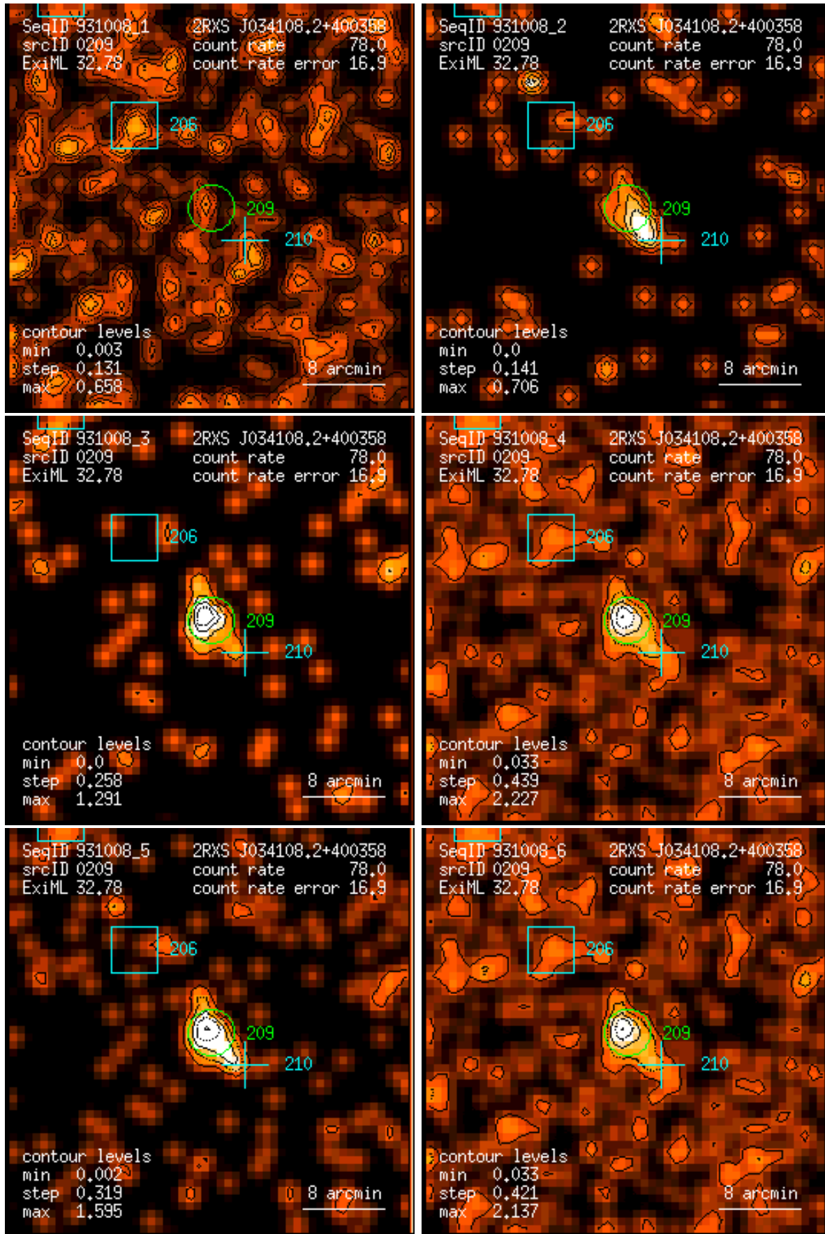
Figure 209: RASS 931008: detection 0209: band rate images, Gaussian filter: (1) PSPC channels 11 – 41, (2) 52 – 90, (3) 91 – 201, (4) 11 – 235, (5) 52 – 201, (6) 11 – 201. Broad band rates in counts/ks. Band rate contour levels in counts/ks/arcmin 2 .
