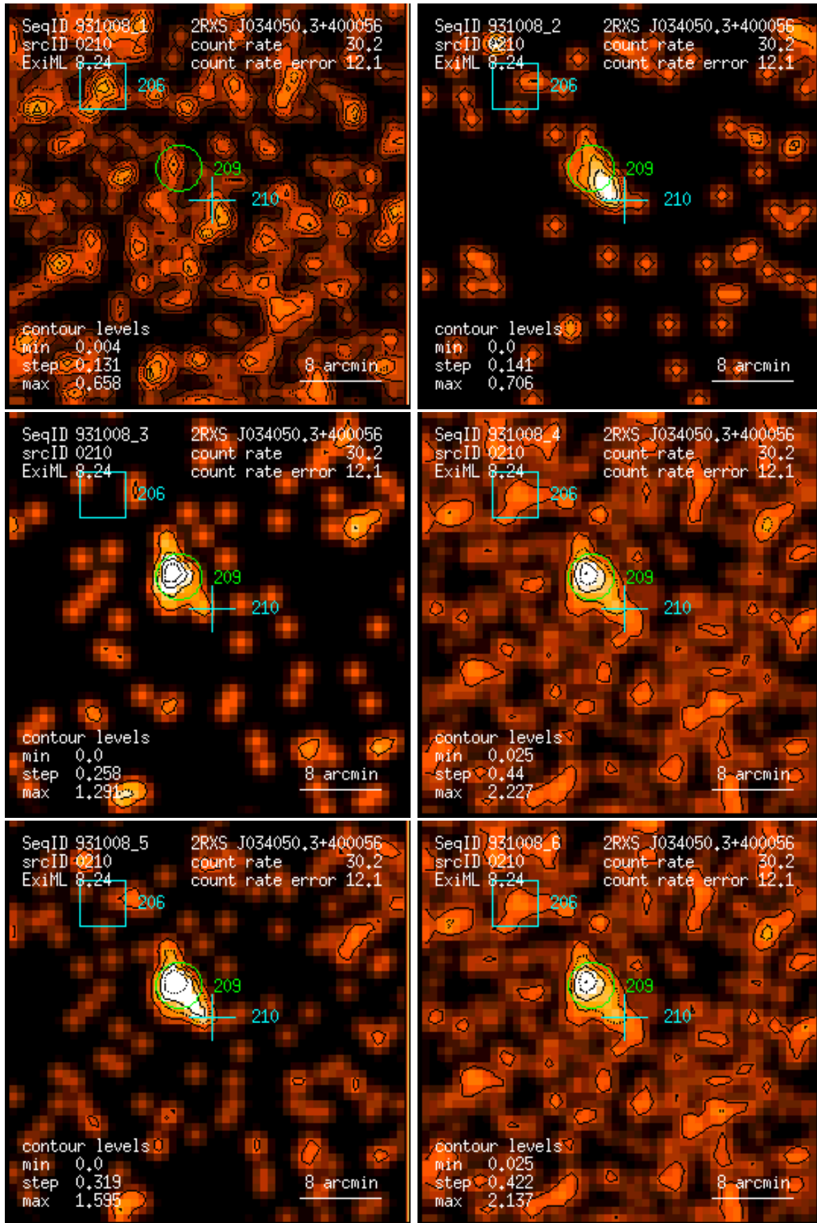
Figure 210: RASS 931008: detection 0210: band rate images, Gaussian filter: (1) PSPC channels 11 – 41, (2) 52 – 90, (3) 91 – 201, (4) 11 – 235, (5) 52 – 201, (6) 11 – 201. Broad band rates in counts/ks. Band rate contour levels in counts/ks/arcmin 2 .
