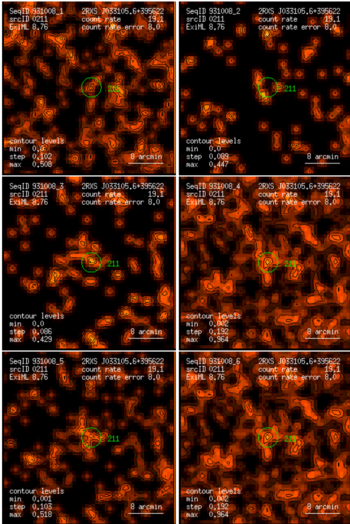
Figure 211: RASS 931008: detection 0211: band rate images, Gaussian filter: (1) PSPC channels 11 – 41, (2) 52 – 90, (3) 91 – 201, (4) 11 – 235, (5) 52 – 201, (6) 11 – 201. Broad band rates in counts/ks. Band rate contour levels in counts/ks/arcmin 2 .
