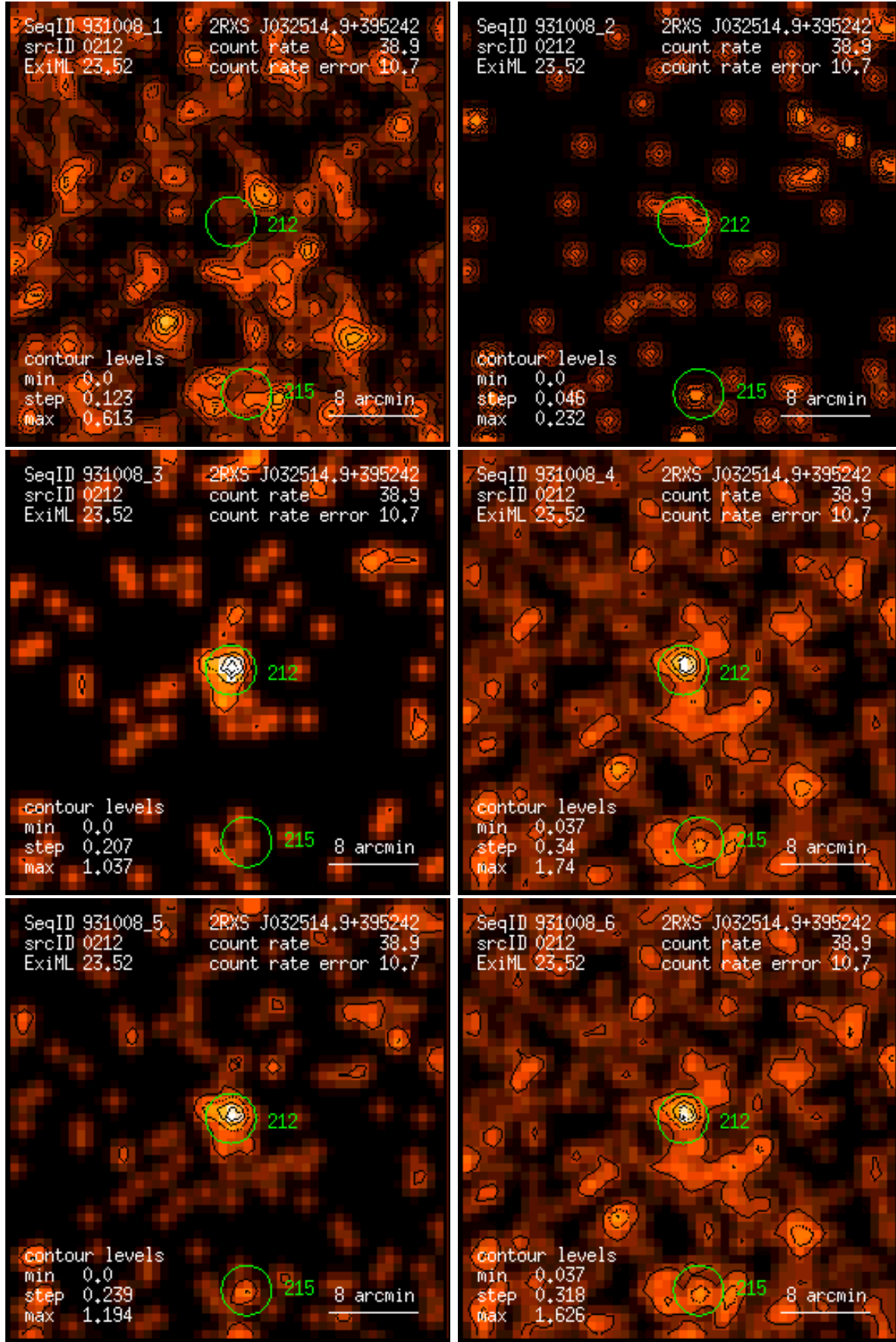
Figure 212: RASS 931008: detection 0212: band rate images, Gaussian filter: (1) PSPC channels 11 – 41, (2) 52 – 90, (3) 91 – 201, (4) 11 – 235, (5) 52 – 201, (6) 11 – 201. Broad band rates in counts/ks. Band rate contour levels in counts/ks/arcmin 2 .
