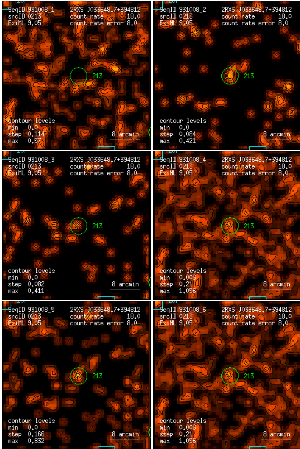
Figure 213: RASS 931008: detection 0213: band rate images, Gaussian filter: (1) PSPC channels 11 – 41, (2) 52 – 90, (3) 91 – 201, (4) 11 – 235, (5) 52 – 201, (6) 11 – 201. Broad band rates in counts/ks. Band rate contour levels in counts/ks/arcmin 2 .
