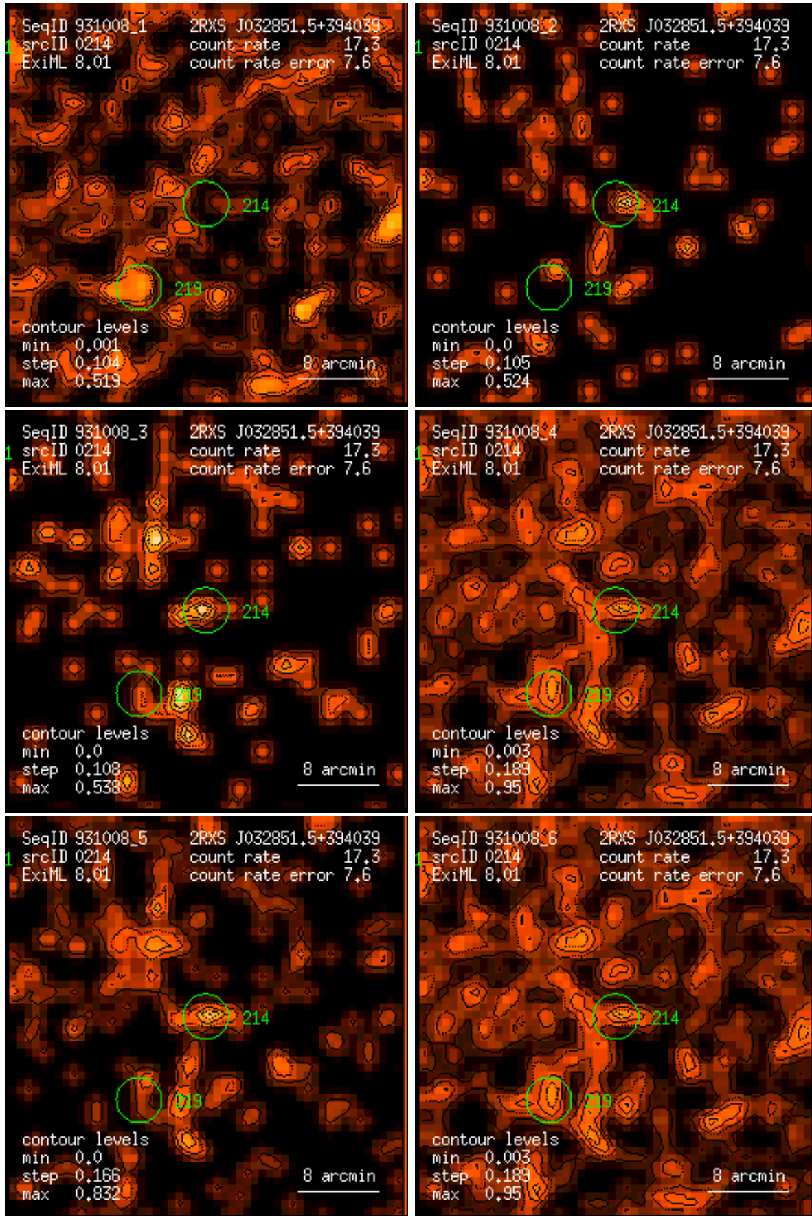
Figure 214: RASS 931008: detection 0214: band rate images, Gaussian filter: (1) PSPC channels 11 – 41, (2) 52 – 90, (3) 91 – 201, (4) 11 – 235, (5) 52 – 201, (6) 11 – 201. Broad band rates in counts/ks. Band rate contour levels in counts/ks/arcmin 2 .
