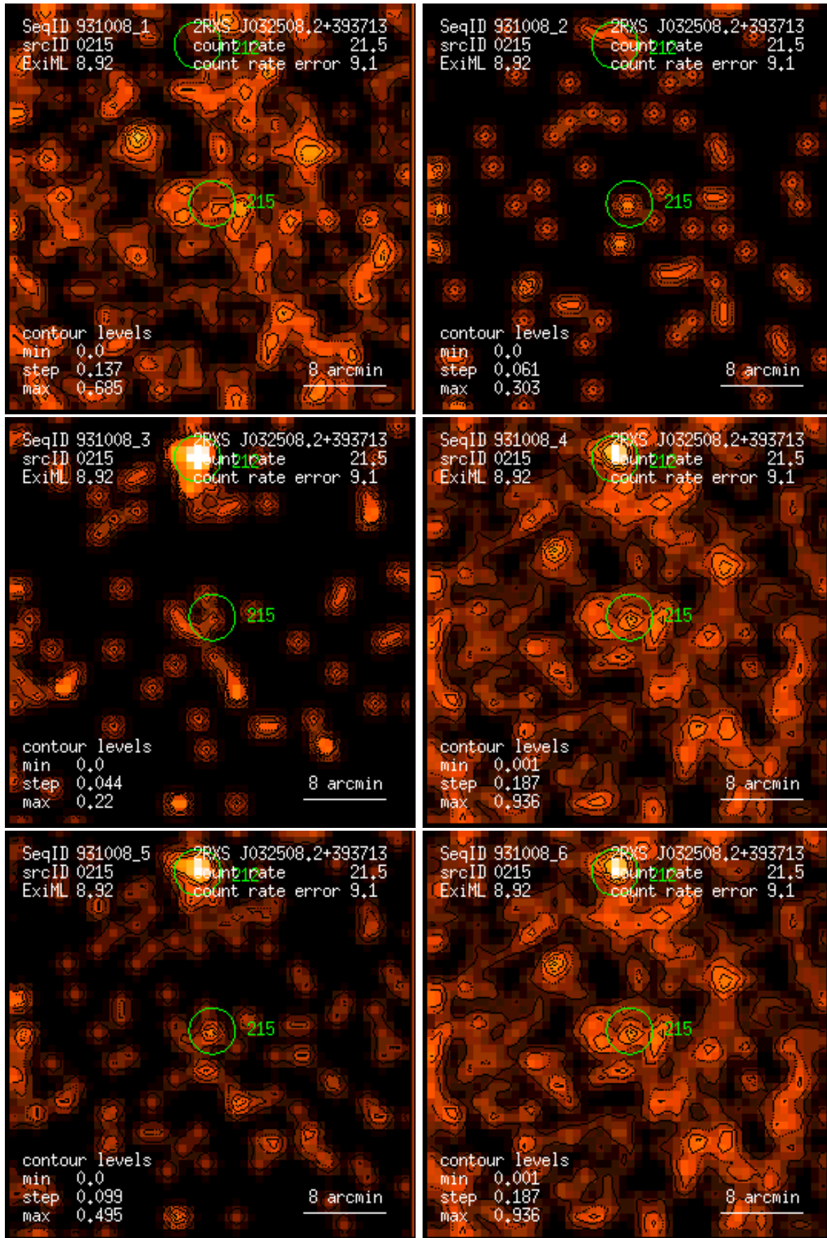
Figure 215: RASS 931008: detection 0215: band rate images, Gaussian filter: (1) PSPC channels 11 – 41, (2) 52 – 90, (3) 91 – 201, (4) 11 – 235, (5) 52 – 201, (6) 11 – 201. Broad band rates in counts/ks. Band rate contour levels in counts/ks/arcmin 2 .
