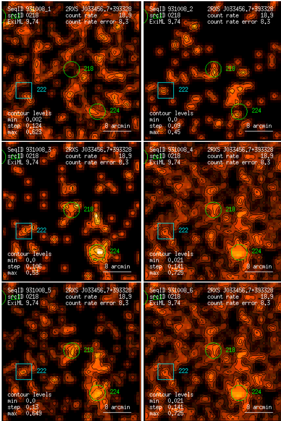
Figure 218: RASS 931008: detection 0218: band rate images, Gaussian filter: (1) PSPC channels 11 – 41, (2) 52 – 90, (3) 91 – 201, (4) 11 – 235, (5) 52 – 201, (6) 11 – 201. Broad band rates in counts/ks. Band rate contour levels in counts/ks/arcmin 2 .
