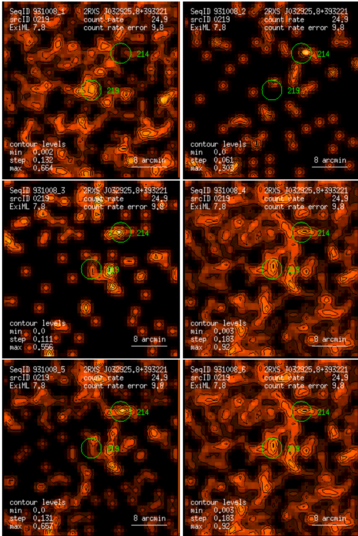
Figure 219: RASS 931008: detection 0219: band rate images, Gaussian filter: (1) PSPC channels 11 – 41, (2) 52 – 90, (3) 91 – 201, (4) 11 – 235, (5) 52 – 201, (6) 11 – 201. Broad band rates in counts/ks. Band rate contour levels in counts/ks/arcmin 2 .
