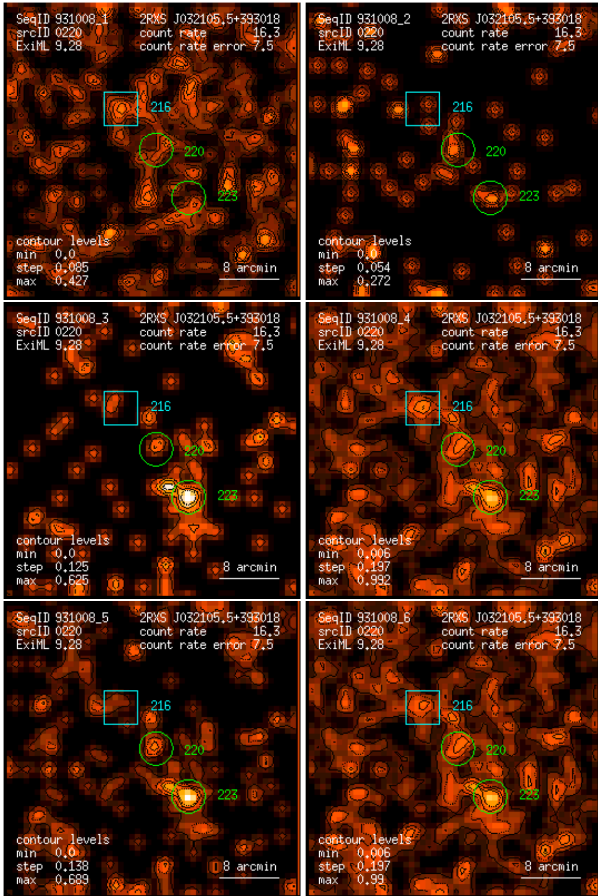
Figure 220: RASS 931008: detection 0220: band rate images, Gaussian filter: (1) PSPC channels 11 – 41, (2) 52 – 90, (3) 91 – 201, (4) 11 – 235, (5) 52 – 201, (6) 11 – 201. Broad band rates in counts/ks. Band rate contour levels in counts/ks/arcmin 2 .
