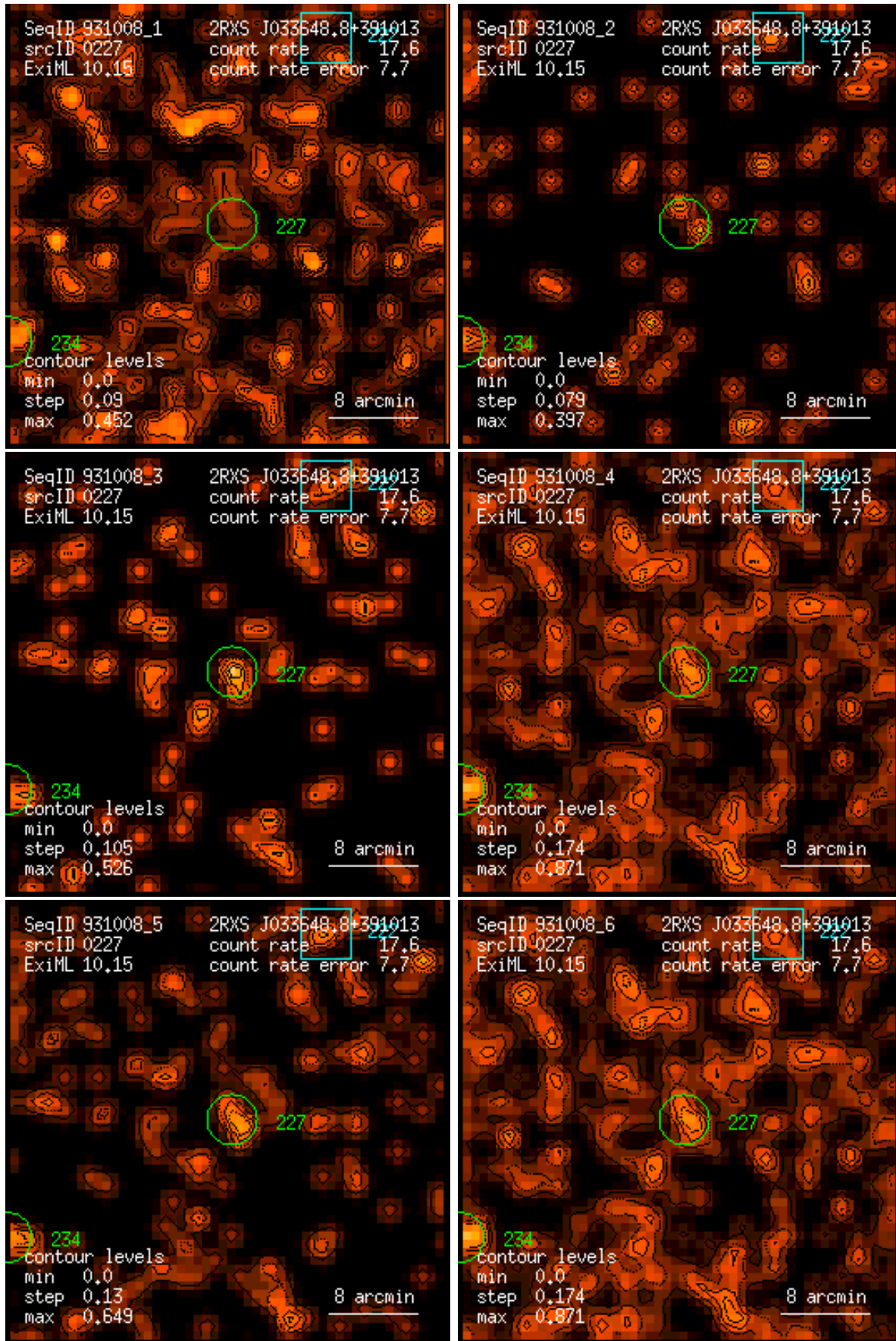
Figure 227: RASS 931008: detection 0227: band rate images, Gaussian filter: (1) PSPC channels 11 – 41, (2) 52 – 90, (3) 91 – 201, (4) 11 – 235, (5) 52 – 201, (6) 11 – 201. Broad band rates in counts/ks. Band rate contour levels in counts/ks/arcmin 2 .
