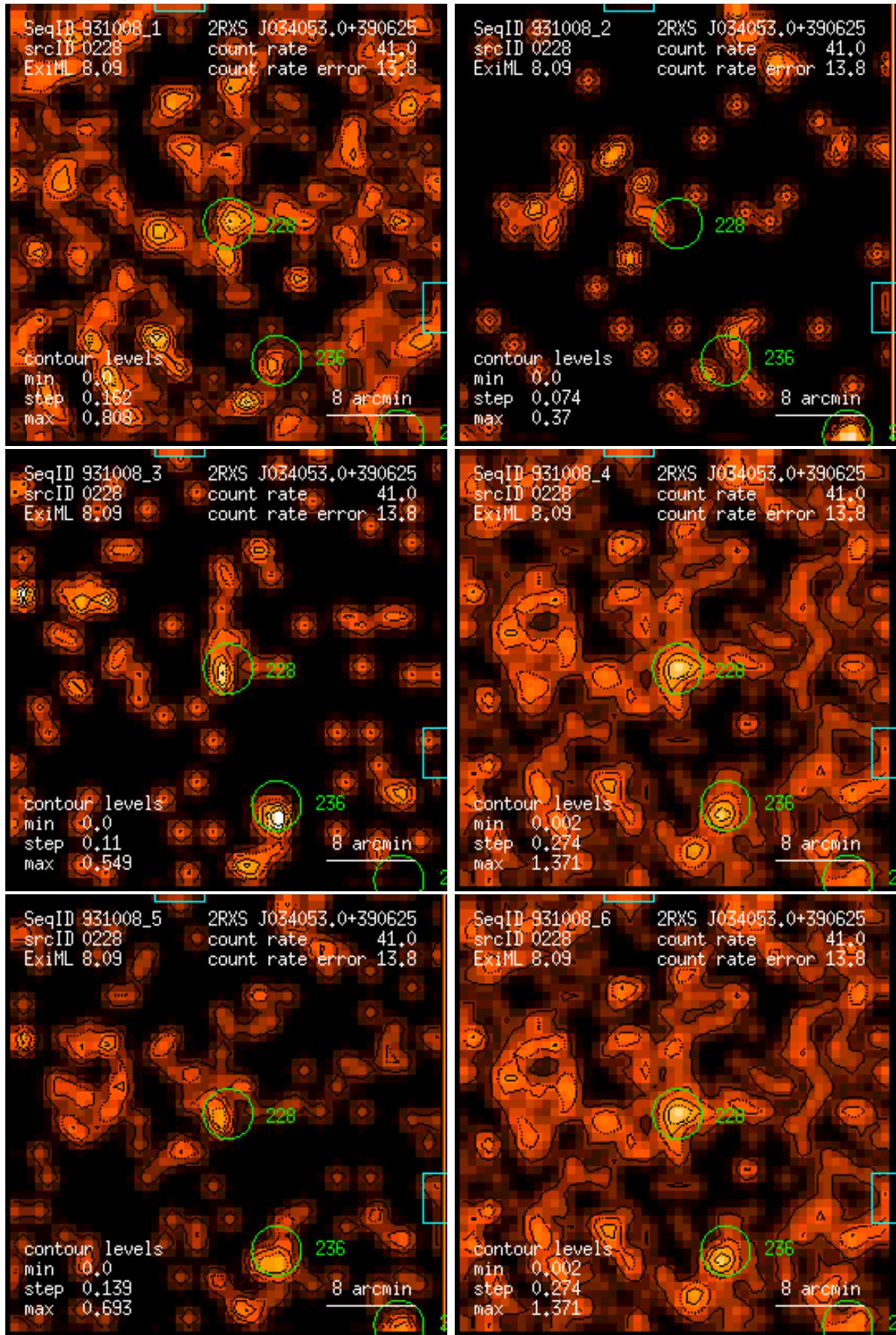
Figure 228: RASS 931008: detection 0228: band rate images, Gaussian filter: (1) PSPC channels 11 – 41, (2) 52 – 90, (3) 91 – 201, (4) 11 – 235, (5) 52 – 201, (6) 11 – 201. Broad band rates in counts/ks. Band rate contour levels in counts/ks/arcmin 2 .
