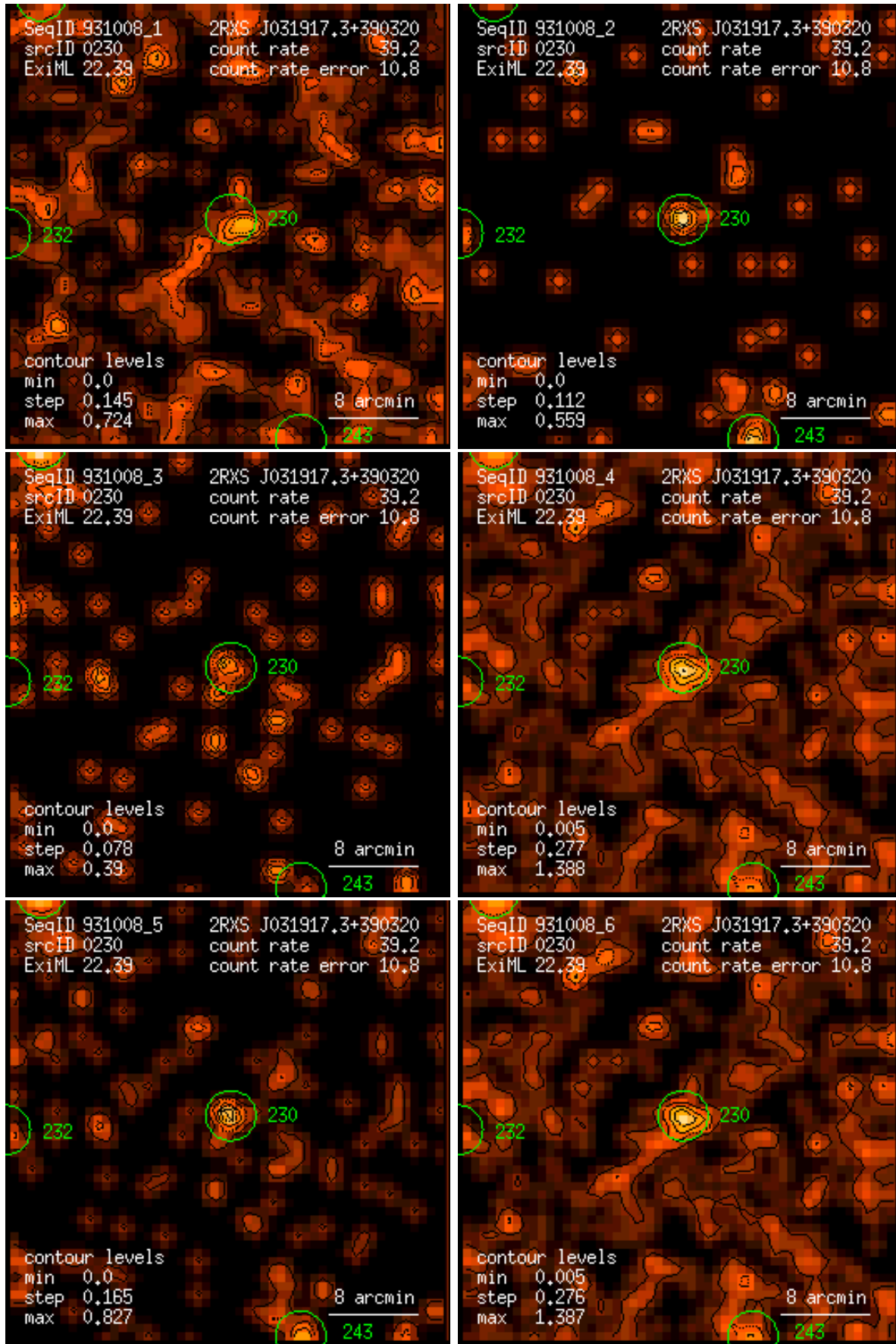
Figure 230: RASS 931008: detection 0230: band rate images, Gaussian filter: (1) PSPC channels 11 – 41, (2) 52 – 90, (3) 91 – 201, (4) 11 – 235, (5) 52 – 201, (6) 11 – 201. Broad band rates in counts/ks. Band rate contour levels in counts/ks/arcmin 2 .
