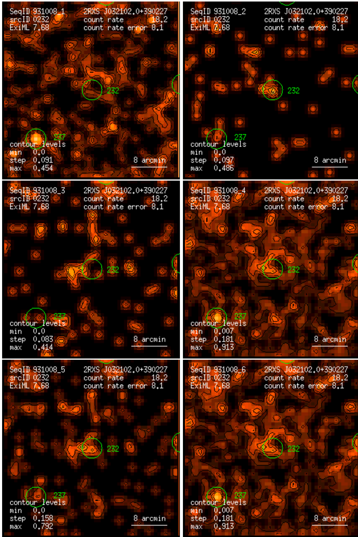
Figure 232: RASS 931008: detection 0232: band rate images, Gaussian filter: (1) PSPC channels 11 – 41, (2) 52 – 90, (3) 91 – 201, (4) 11 – 235, (5) 52 – 201, (6) 11 – 201. Broad band rates in counts/ks. Band rate contour levels in counts/ks/arcmin 2 .
