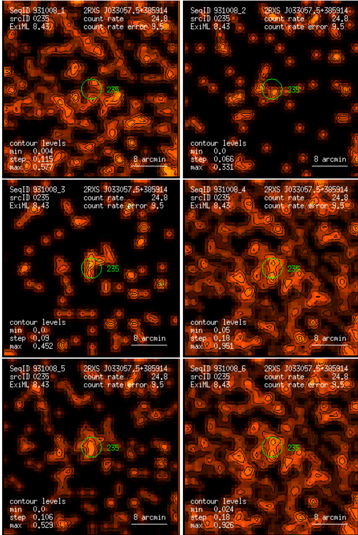
Figure 235: RASS 931008: detection 0235: band rate images, Gaussian filter: (1) PSPC channels 11 – 41, (2) 52 – 90, (3) 91 – 201, (4) 11 – 235, (5) 52 – 201, (6) 11 – 201. Broad band rates in counts/ks. Band rate contour levels in counts/ks/arcmin 2 .
