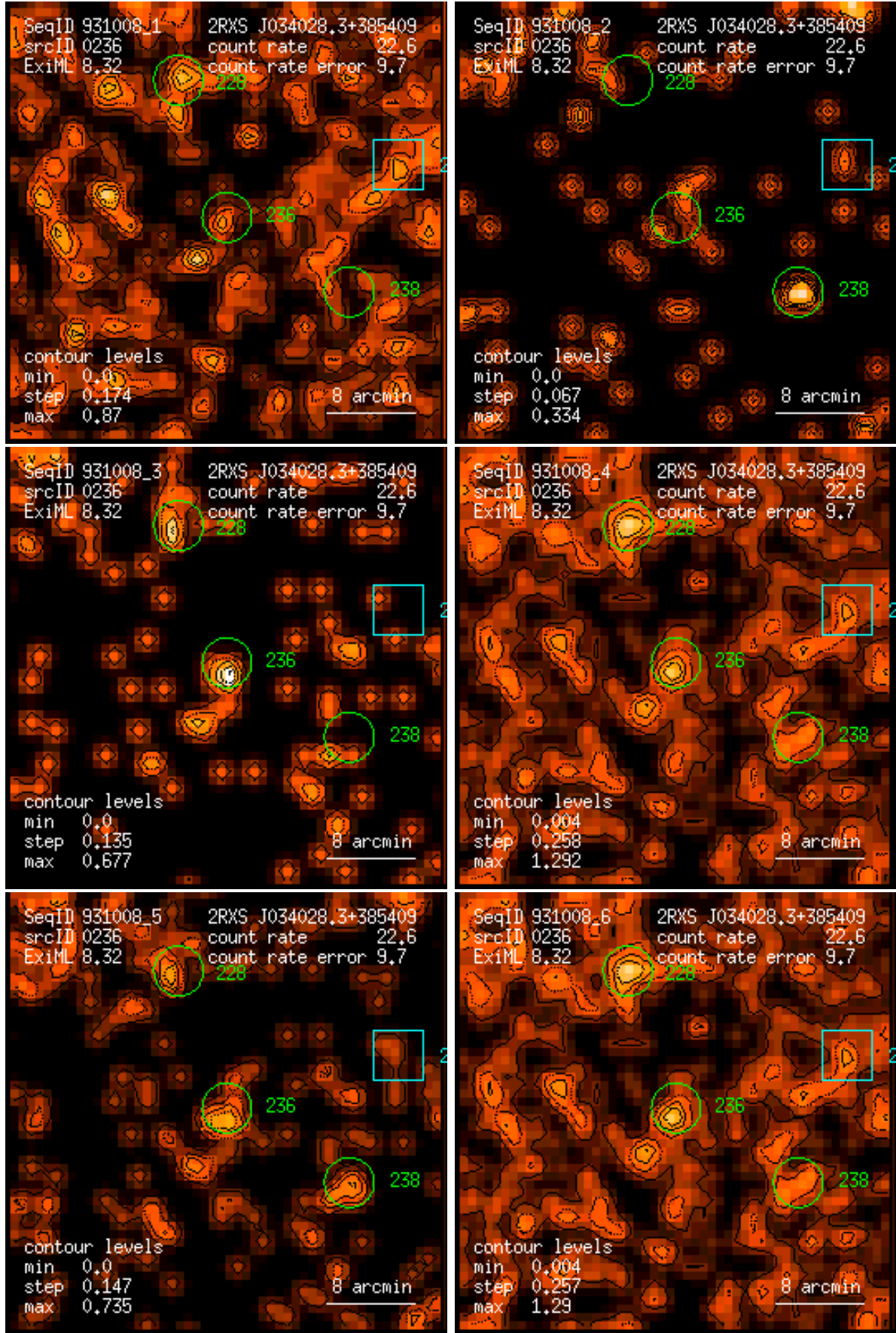
Figure 236: RASS 931008: detection 0236: band rate images, Gaussian filter: (1) PSPC channels 11 – 41, (2) 52 – 90, (3) 91 – 201, (4) 11 – 235, (5) 52 – 201, (6) 11 – 201. Broad band rates in counts/ks. Band rate contour levels in counts/ks/arcmin 2 .
