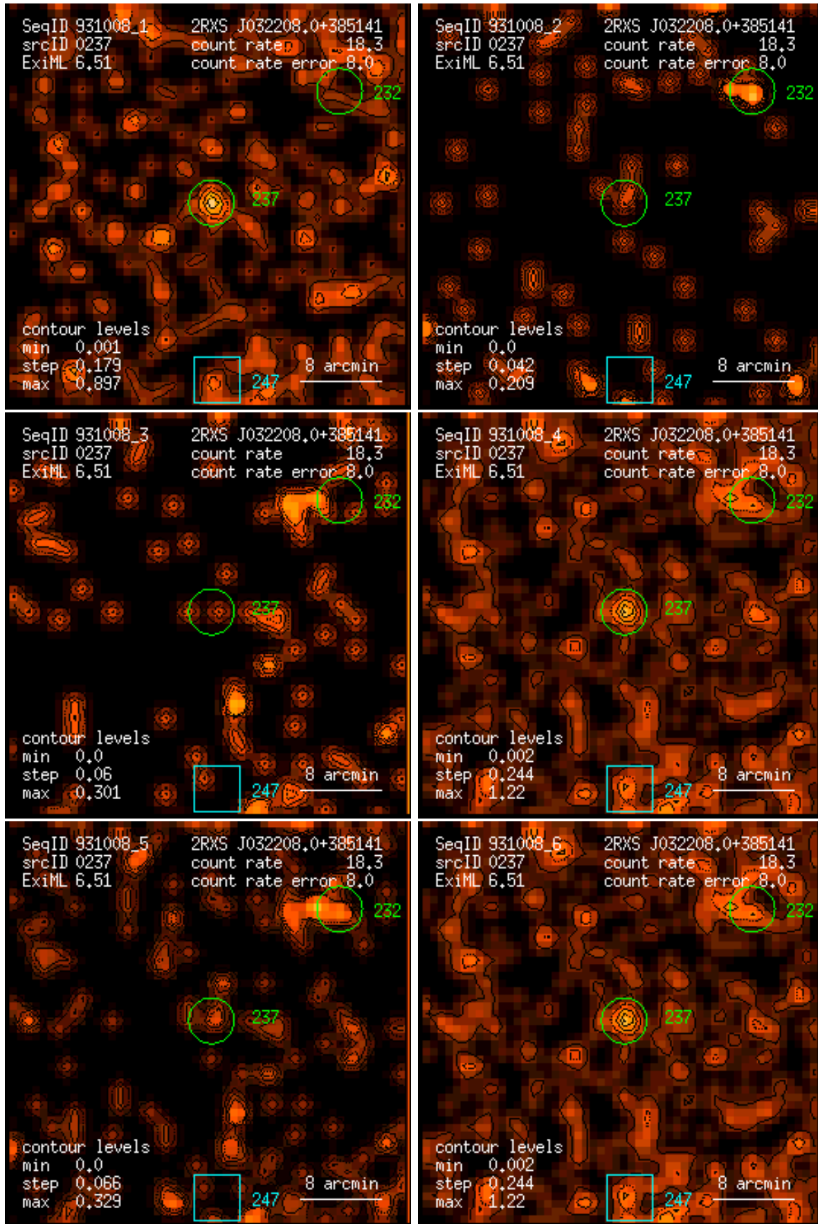
Figure 237: RASS 931008: detection 0237: band rate images, Gaussian filter: (1) PSPC channels 11 – 41, (2) 52 – 90, (3) 91 – 201, (4) 11 – 235, (5) 52 – 201, (6) 11 – 201. Broad band rates in counts/ks. Band rate contour levels in counts/ks/arcmin 2 .
