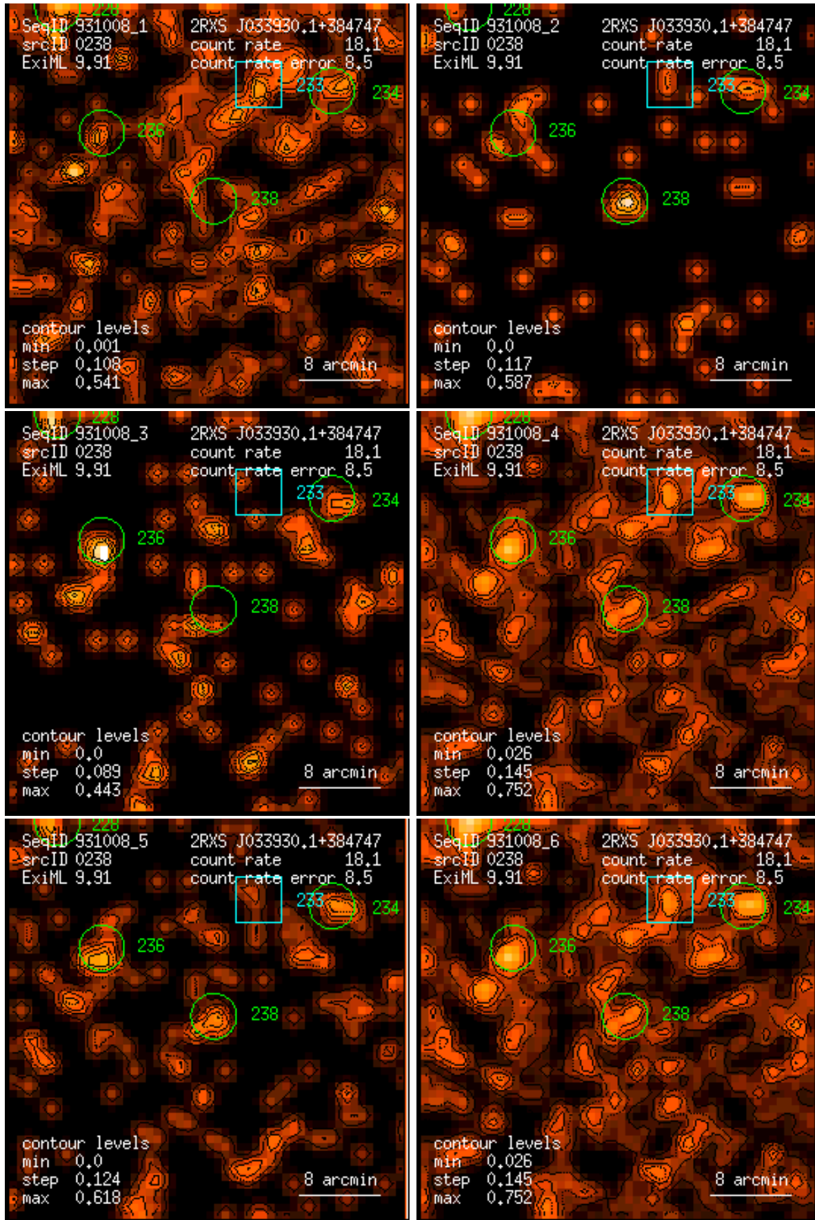
Figure 238: RASS 931008: detection 0238: band rate images, Gaussian filter: (1) PSPC channels 11 – 41, (2) 52 – 90, (3) 91 – 201, (4) 11 – 235, (5) 52 – 201, (6) 11 – 201. Broad band rates in counts/ks. Band rate contour levels in counts/ks/arcmin 2 .
