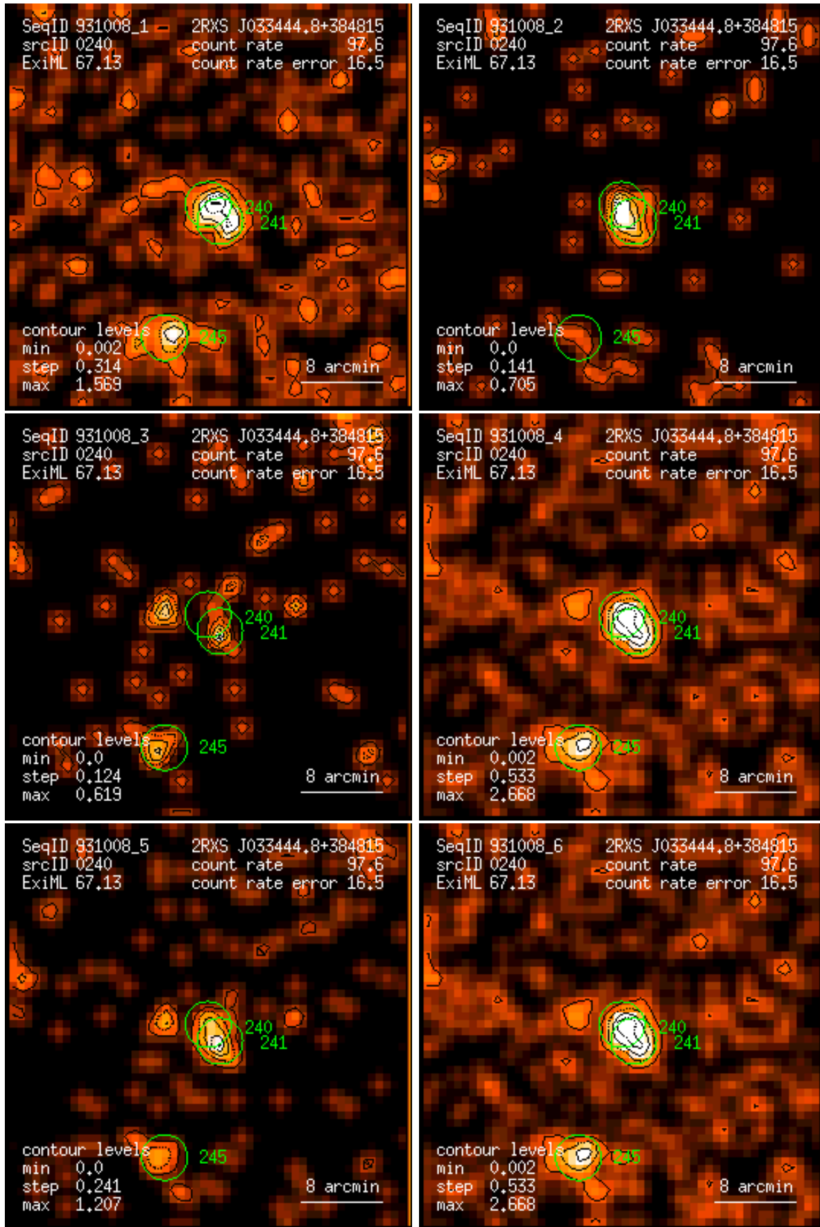
Figure 240: RASS 931008: detection 0240: band rate images, Gaussian filter: (1) PSPC channels 11 – 41, (2) 52 – 90, (3) 91 – 201, (4) 11 – 235, (5) 52 – 201, (6) 11 – 201. Broad band rates in counts/ks. Band rate contour levels in counts/ks/arcmin 2 .
