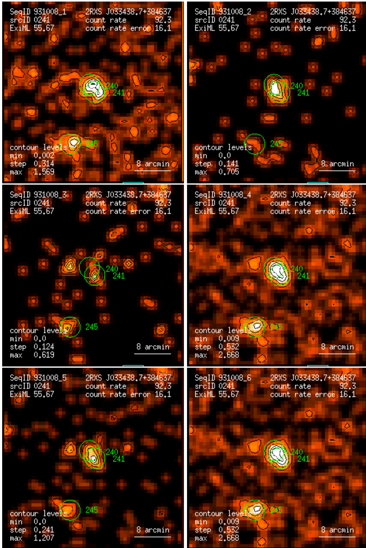
Figure 241: RASS 931008: detection 0241: band rate images, Gaussian filter: (1) PSPC channels 11 – 41, (2) 52 – 90, (3) 91 – 201, (4) 11 – 235, (5) 52 – 201, (6) 11 – 201. Broad band rates in counts/ks. Band rate contour levels in counts/ks/arcmin 2 .
