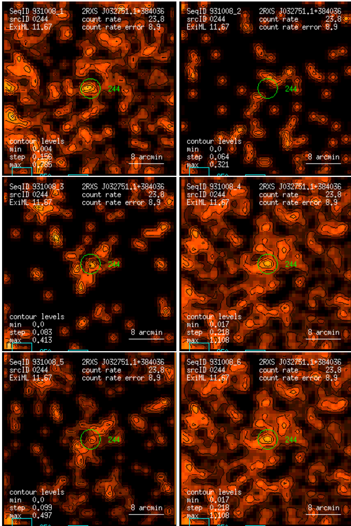
Figure 244: RASS 931008: detection 0244: band rate images, Gaussian filter: (1) PSPC channels 11 – 41, (2) 52 – 90, (3) 91 – 201, (4) 11 – 235, (5) 52 – 201, (6) 11 – 201. Broad band rates in counts/ks. Band rate contour levels in counts/ks/arcmin 2 .
