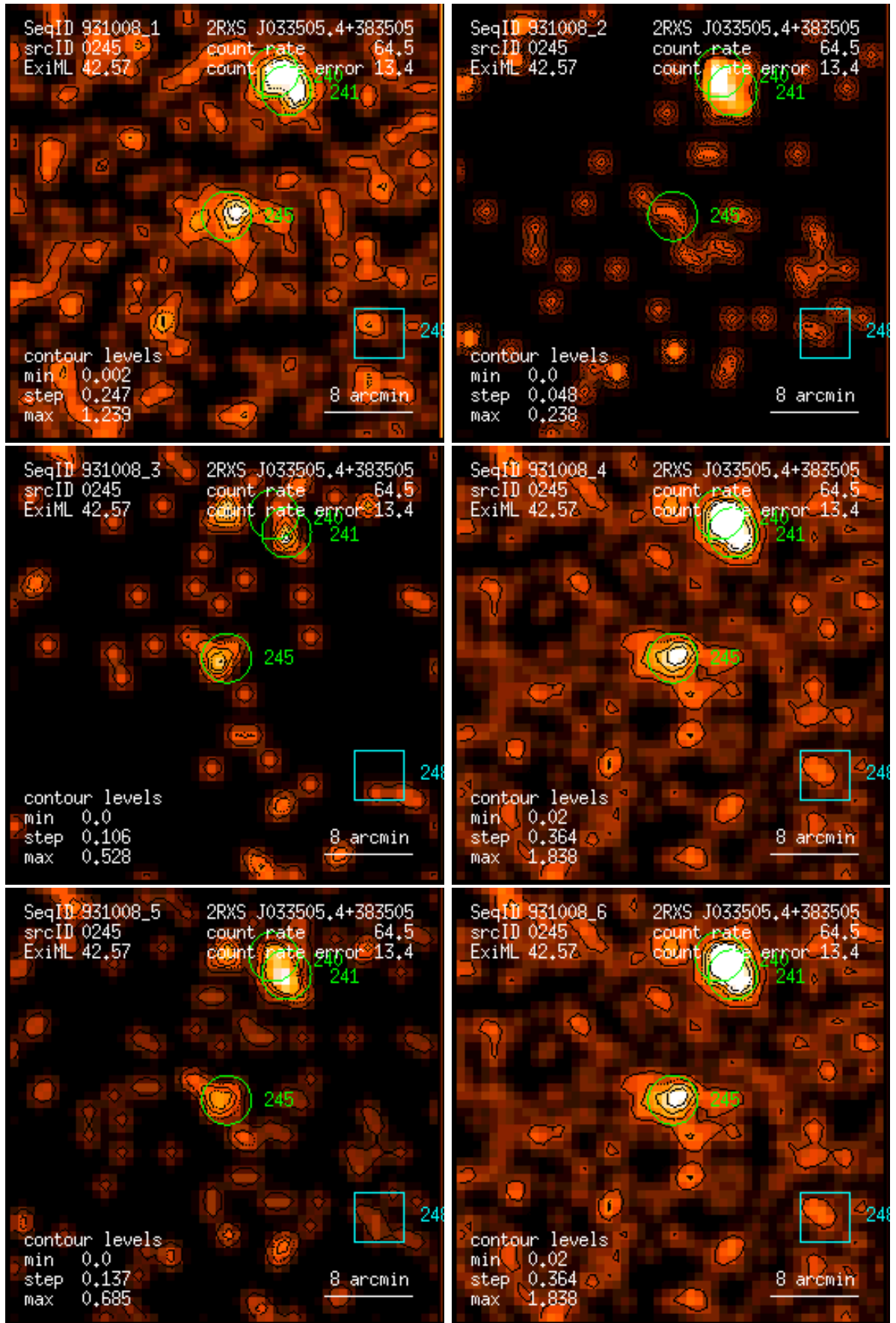
Figure 245: RASS 931008: detection 0245: band rate images, Gaussian filter: (1) PSPC channels 11 – 41, (2) 52 – 90, (3) 91 – 201, (4) 11 – 235, (5) 52 – 201, (6) 11 – 201. Broad band rates in counts/ks. Band rate contour levels in counts/ks/arcmin 2 .
