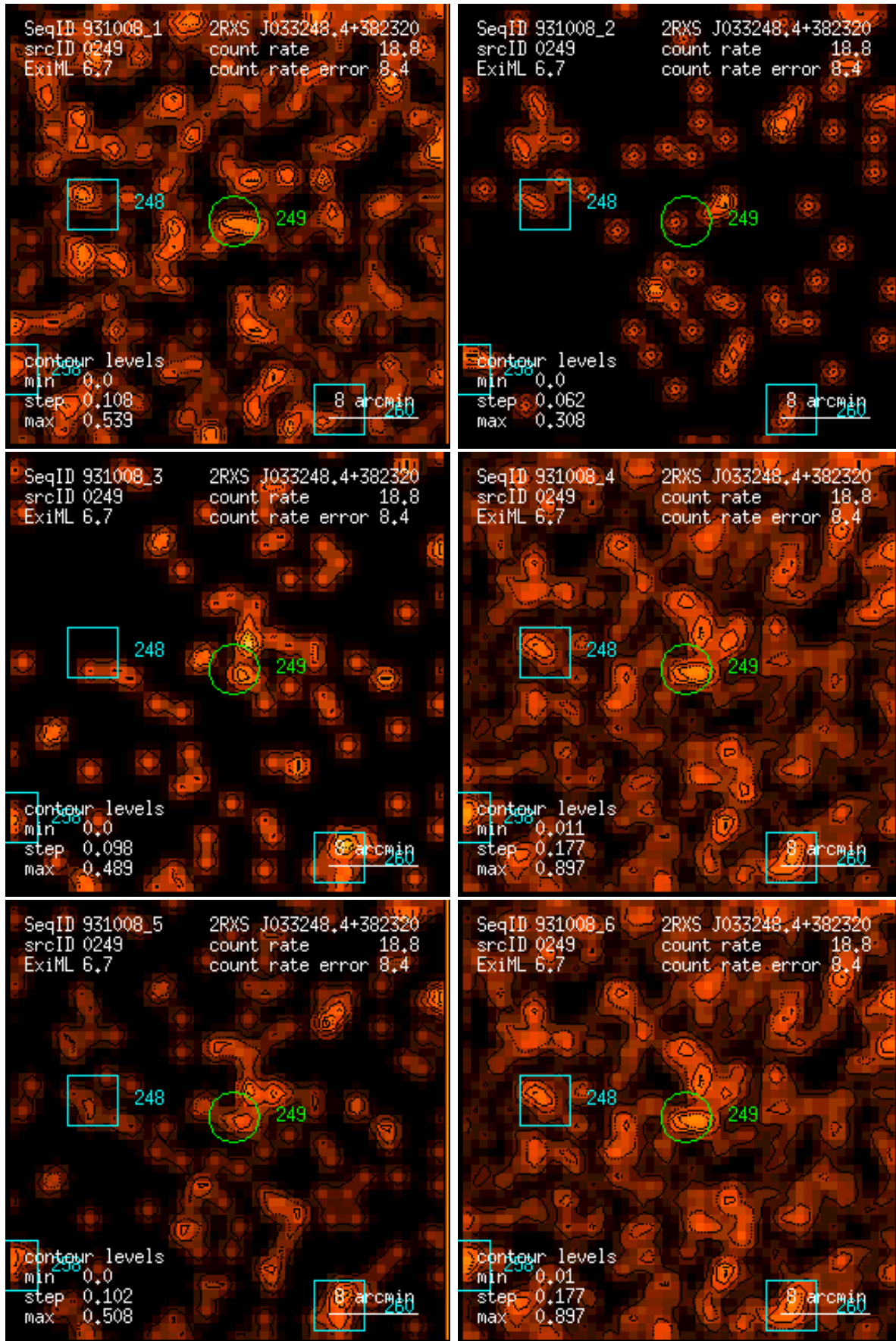
Figure 249: RASS 931008: detection 0249: band rate images, Gaussian filter: (1) PSPC channels 11 – 41, (2) 52 – 90, (3) 91 – 201, (4) 11 – 235, (5) 52 – 201, (6) 11 – 201. Broad band rates in counts/ks. Band rate contour levels in counts/ks/arcmin 2 .
