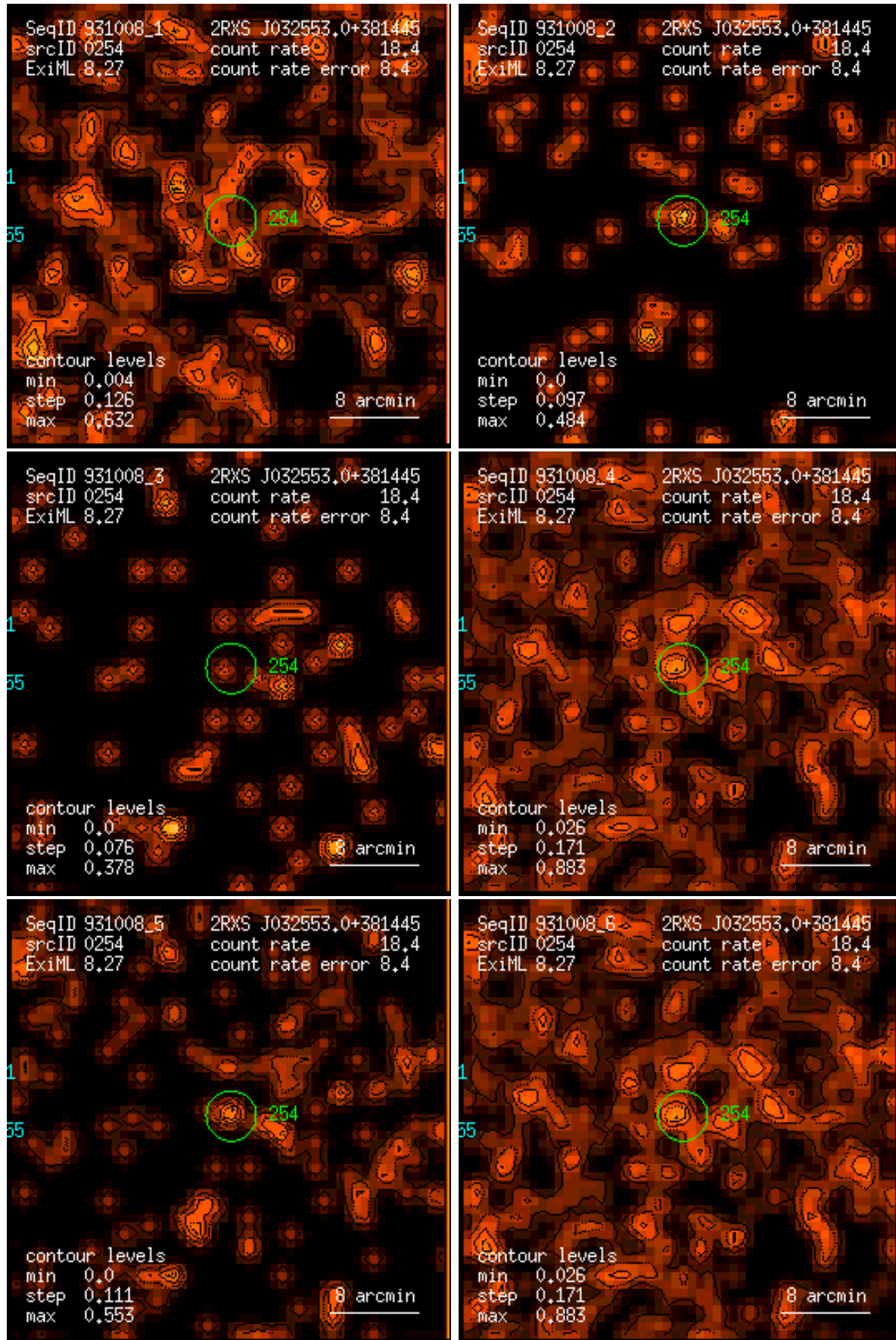
Figure 254: RASS 931008: detection 0254: band rate images, Gaussian filter: (1) PSPC channels 11 – 41, (2) 52 – 90, (3) 91 – 201, (4) 11 – 235, (5) 52 – 201, (6) 11 – 201. Broad band rates in counts/ks. Band rate contour levels in counts/ks/arcmin 2 .
