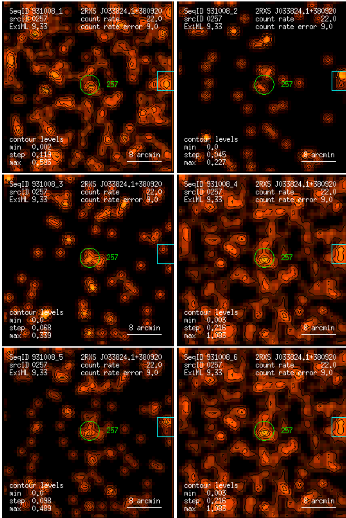
Figure 257: RASS 931008: detection 0257: band rate images, Gaussian filter: (1) PSPC channels 11 – 41, (2) 52 – 90, (3) 91 – 201, (4) 11 – 235, (5) 52 – 201, (6) 11 – 201. Broad band rates in counts/ks. Band rate contour levels in counts/ks/arcmin 2 .
