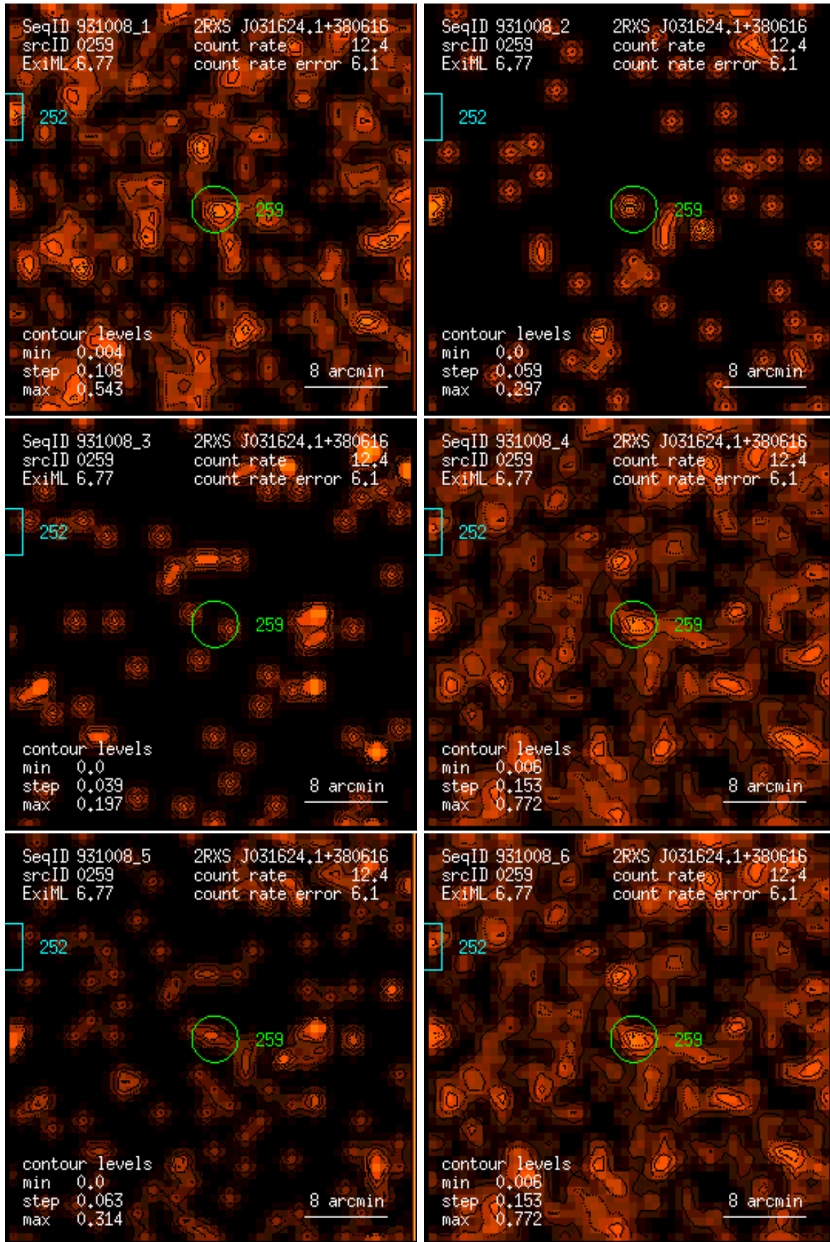
Figure 259: RASS 931008: detection 0259: band rate images, Gaussian filter: (1) PSPC channels 11 – 41, (2) 52 – 90, (3) 91 – 201, (4) 11 – 235, (5) 52 – 201, (6) 11 – 201. Broad band rates in counts/ks. Band rate contour levels in counts/ks/arcmin 2 .
