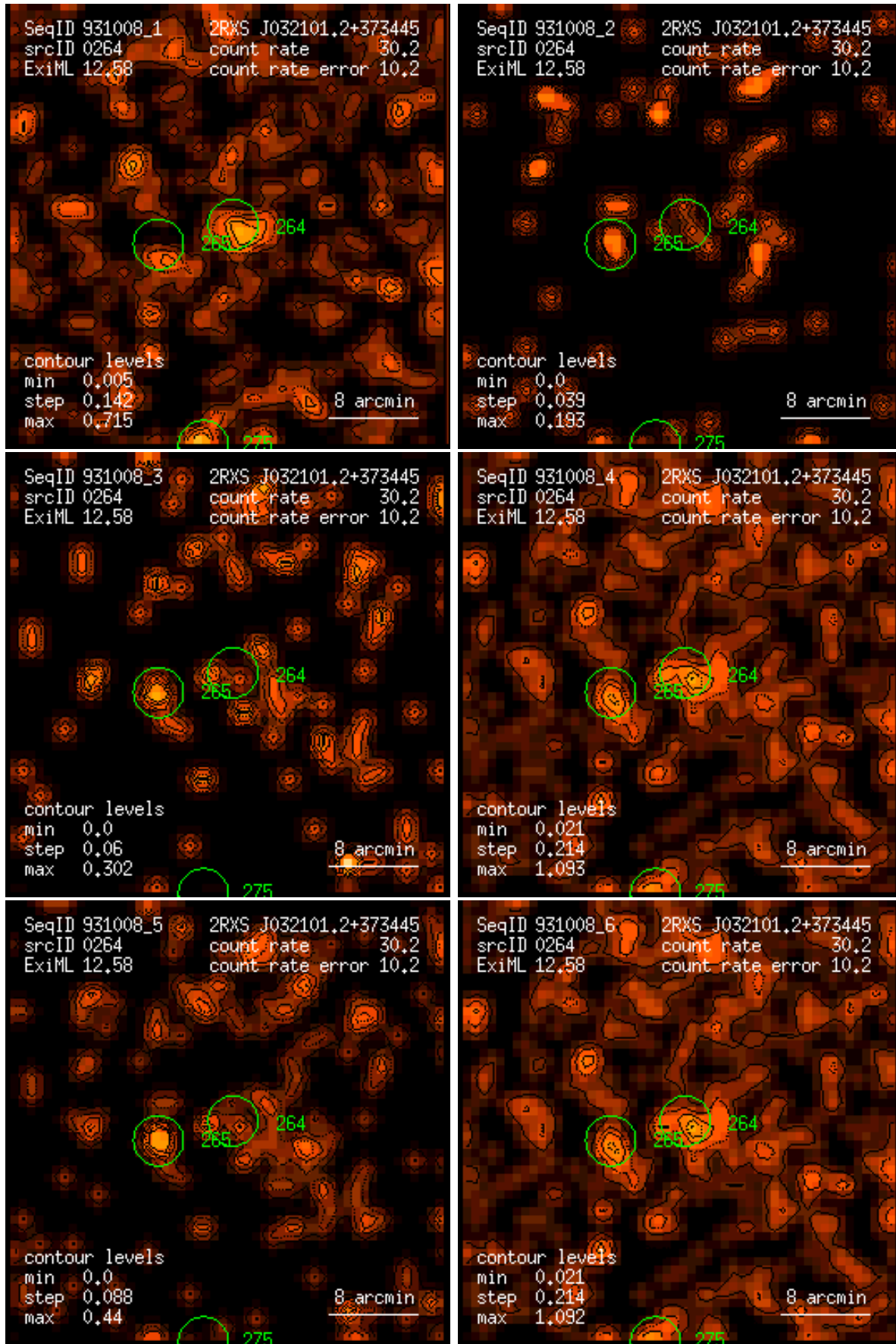
Figure 264: RASS 931008: detection 0264: band rate images, Gaussian filter: (1) PSPC channels 11 – 41, (2) 52 – 90, (3) 91 – 201, (4) 11 – 235, (5) 52 – 201, (6) 11 – 201. Broad band rates in counts/ks. Band rate contour levels in counts/ks/arcmin 2 .
