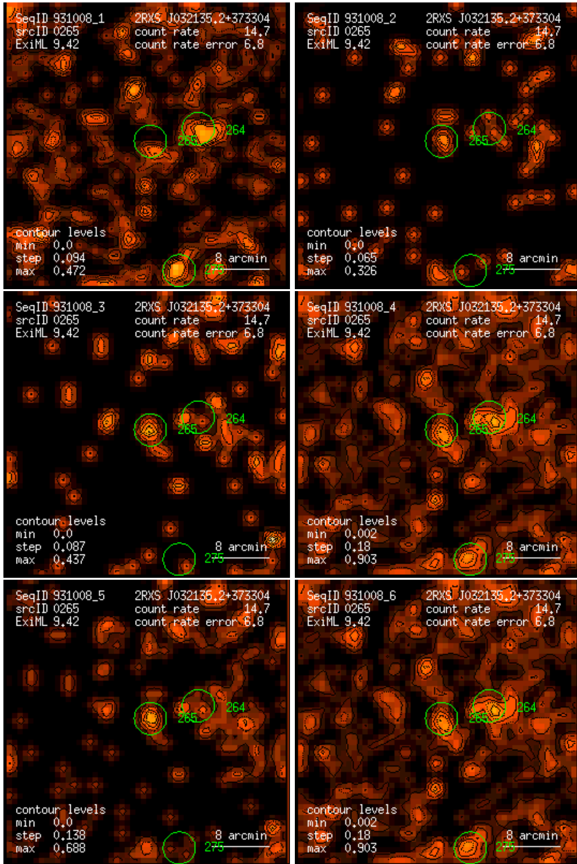
Figure 265: RASS 931008: detection 0265: band rate images, Gaussian filter: (1) PSPC channels 11 – 41, (2) 52 – 90, (3) 91 – 201, (4) 11 – 235, (5) 52 – 201, (6) 11 – 201. Broad band rates in counts/ks. Band rate contour levels in counts/ks/arcmin 2 .
