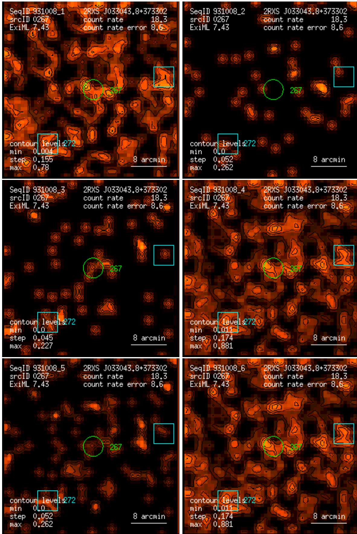
Figure 267: RASS 931008: detection 0267: band rate images, Gaussian filter: (1) PSPC channels 11 – 41, (2) 52 – 90, (3) 91 – 201, (4) 11 – 235, (5) 52 – 201, (6) 11 – 201. Broad band rates in counts/ks. Band rate contour levels in counts/ks/arcmin 2 .
