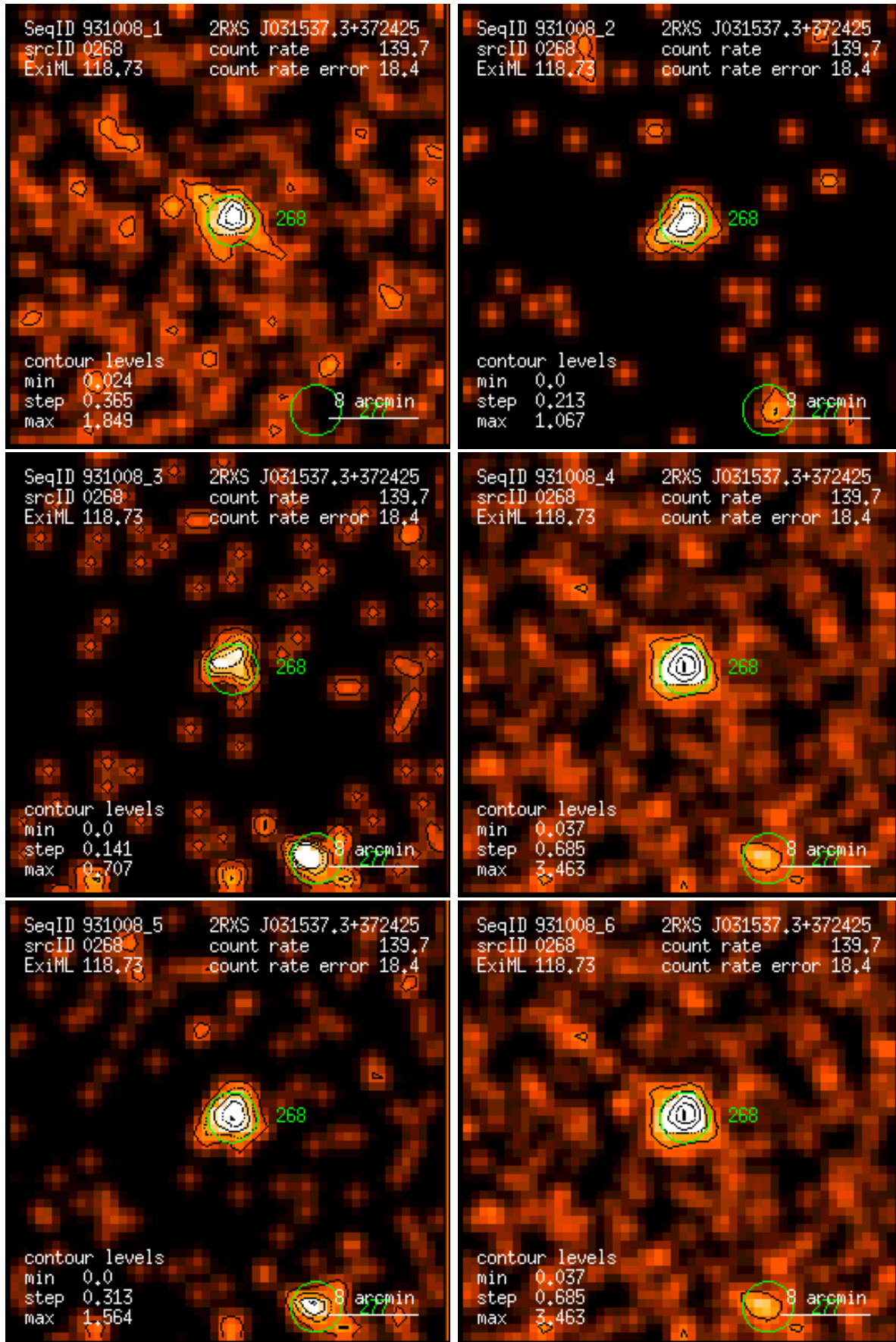
Figure 268: RASS 931008: detection 0268: band rate images, Gaussian filter: (1) PSPC channels 11 – 41, (2) 52 – 90, (3) 91 – 201, (4) 11 – 235, (5) 52 – 201, (6) 11 – 201. Broad band rates in counts/ks. Band rate contour levels in counts/ks/arcmin 2 .
