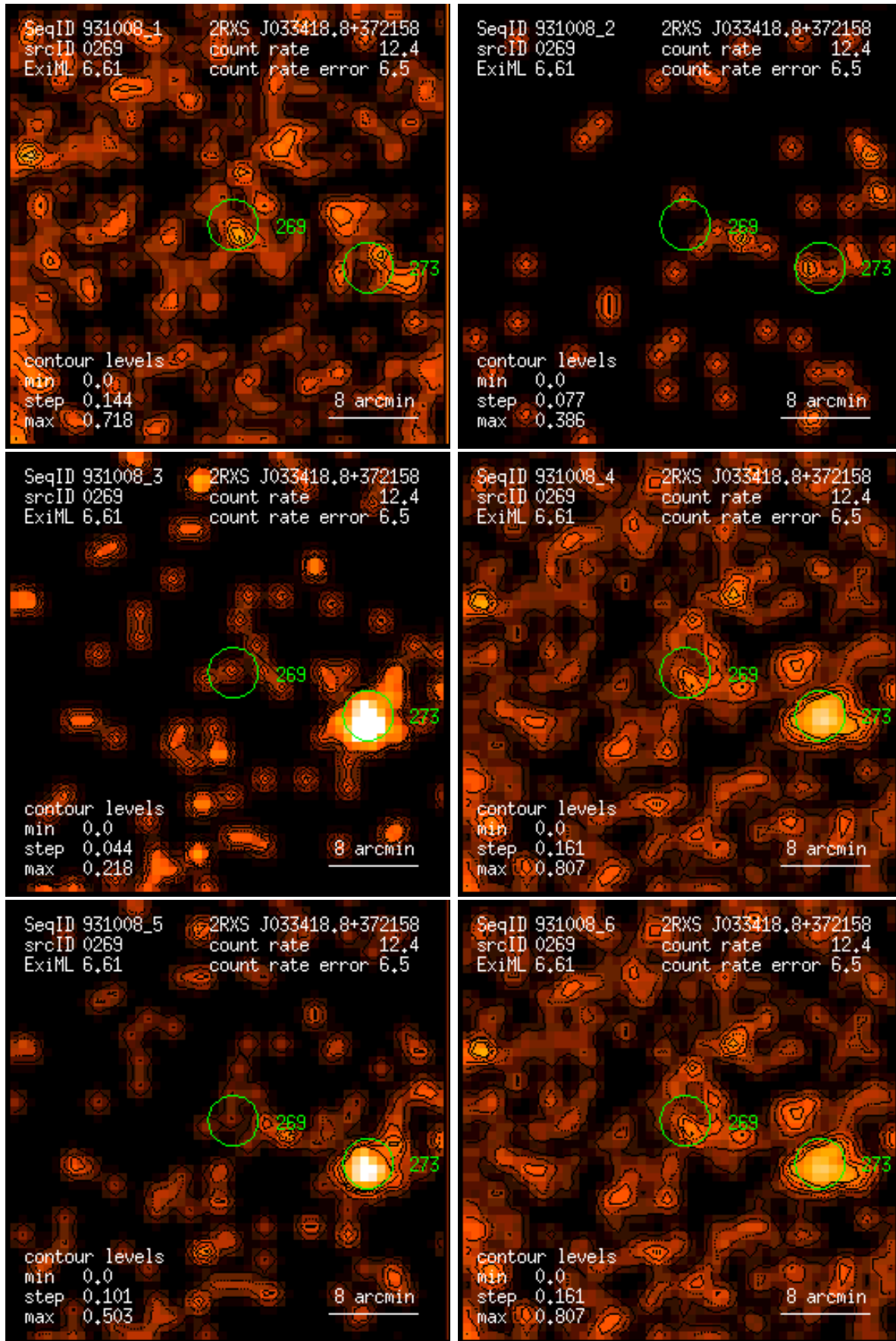
Figure 269: RASS 931008: detection 0269: band rate images, Gaussian filter: (1) PSPC channels 11 – 41, (2) 52 – 90, (3) 91 – 201, (4) 11 – 235, (5) 52 – 201, (6) 11 – 201. Broad band rates in counts/ks. Band rate contour levels in counts/ks/arcmin 2 .
