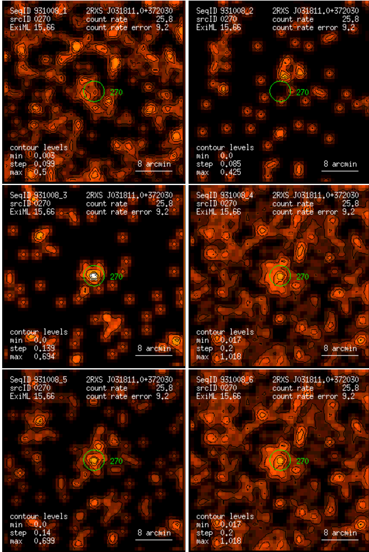
Figure 270: RASS 931008: detection 0270: band rate images, Gaussian filter: (1) PSPC channels 11 – 41, (2) 52 – 90, (3) 91 – 201, (4) 11 – 235, (5) 52 – 201, (6) 11 – 201. Broad band rates in counts/ks. Band rate contour levels in counts/ks/arcmin 2 .
