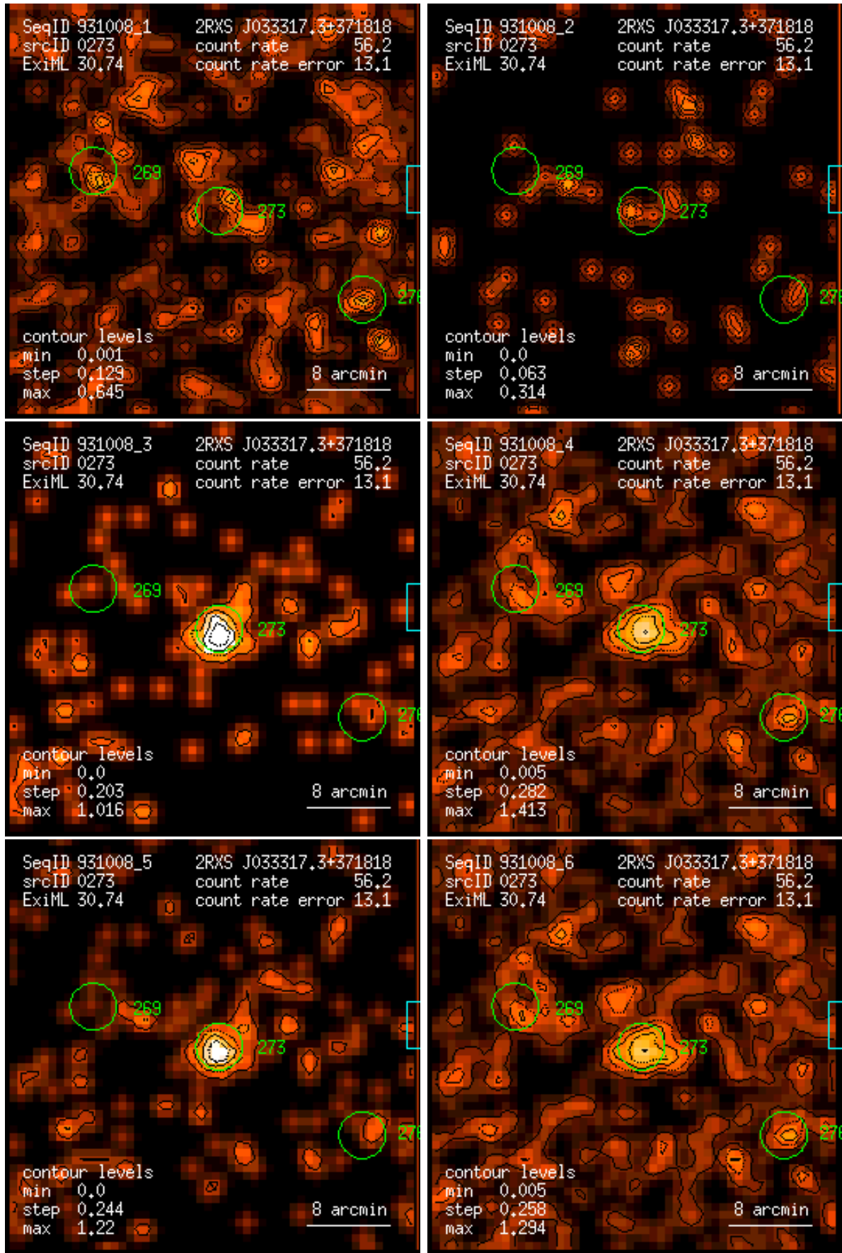
Figure 273: RASS 931008: detection 0273: band rate images, Gaussian filter: (1) PSPC channels 11 – 41, (2) 52 – 90, (3) 91 – 201, (4) 11 – 235, (5) 52 – 201, (6) 11 – 201. Broad band rates in counts/ks. Band rate contour levels in counts/ks/arcmin 2 .
