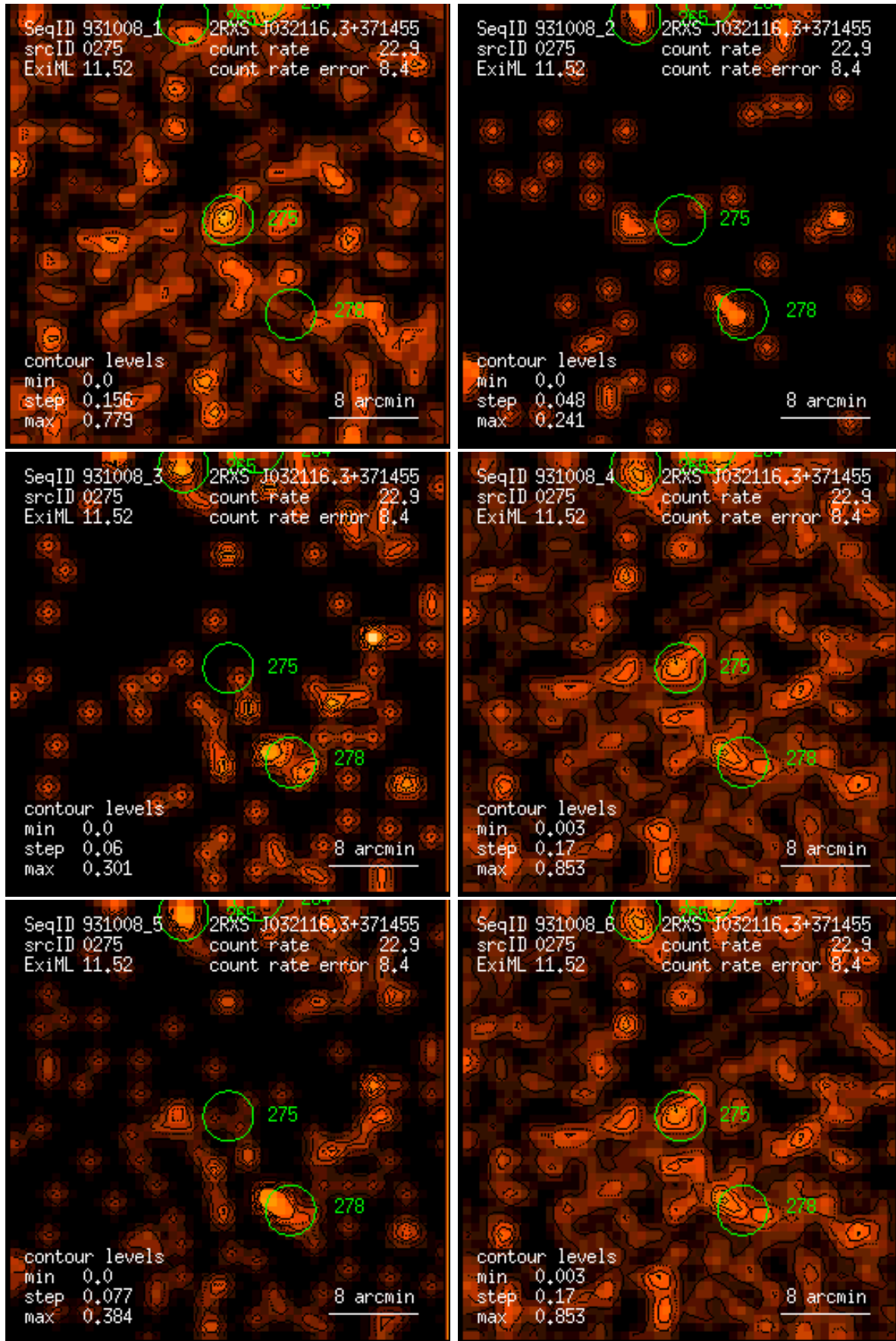
Figure 275: RASS 931008: detection 0275: band rate images, Gaussian filter: (1) PSPC channels 11 – 41, (2) 52 – 90, (3) 91 – 201, (4) 11 – 235, (5) 52 – 201, (6) 11 – 201. Broad band rates in counts/ks. Band rate contour levels in counts/ks/arcmin 2 .
