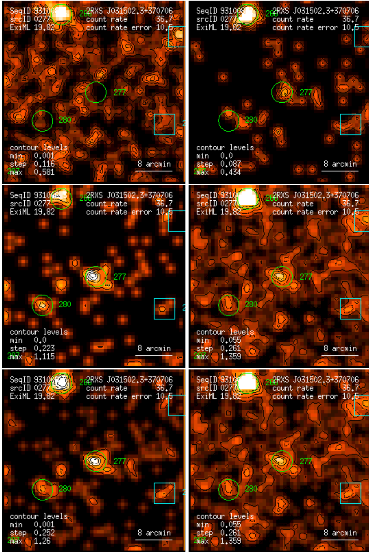
Figure 277: RASS 931008: detection 0277: band rate images, Gaussian filter: (1) PSPC channels 11 – 41, (2) 52 – 90, (3) 91 – 201, (4) 11 – 235, (5) 52 – 201, (6) 11 – 201. Broad band rates in counts/ks. Band rate contour levels in counts/ks/arcmin 2 .
